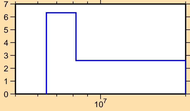
\Delta\sigma/\sigma vs. E for ^{179}\text{Tm}(n,\text{tot.})
