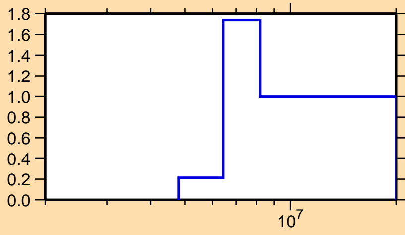
\sigma vs. E for ^{179}\text{Tm}(n,2n)
