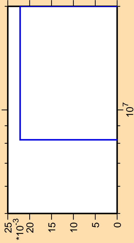
\Delta\sigma/\sigma vs. E for ^{179}\text{Tm} (mt 11)
