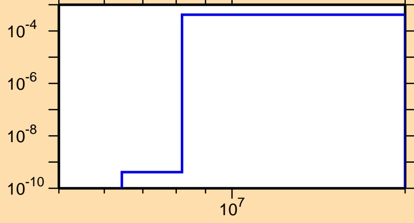
\sigma vs. E for ^{179}\text{Tm}(n,p)
