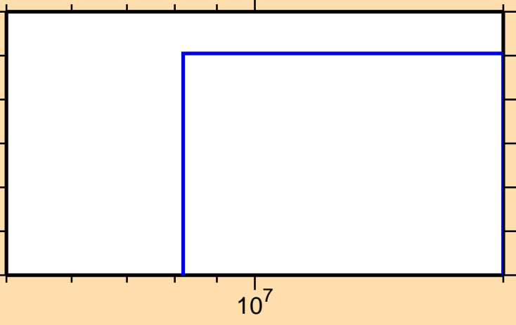
\sigma vs. E for ^{179}\text{Tm}(n,nd)
