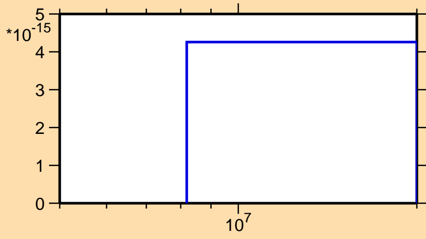
\sigma vs. E for ^{179}\text{Tm} (mt 11)
