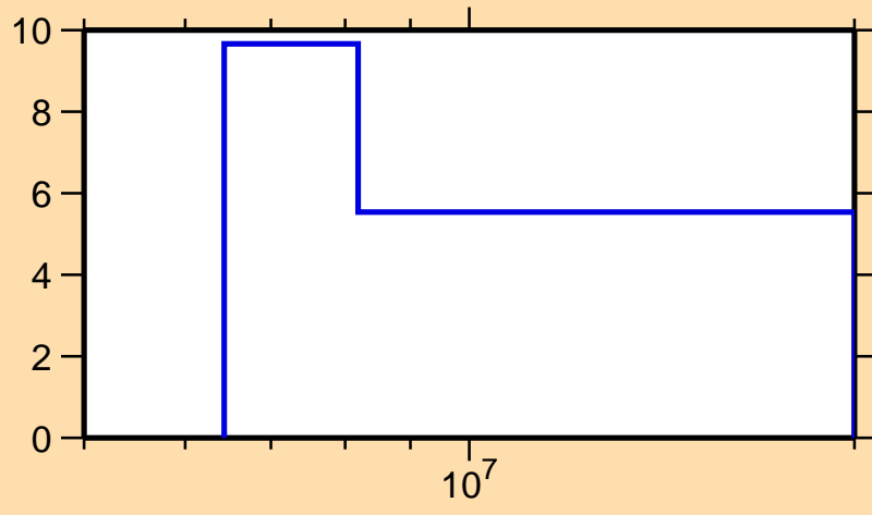
\Delta\sigma/\sigma vs. E for ^{179}\text{Tm}(n,el.)
