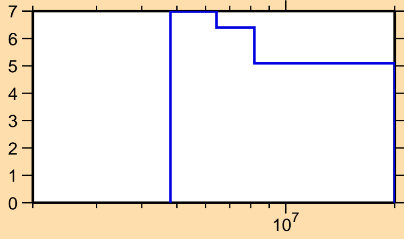
\Delta\sigma/\sigma vs. E for ^{179}\text{Tm}(n,\text{nonel.})
