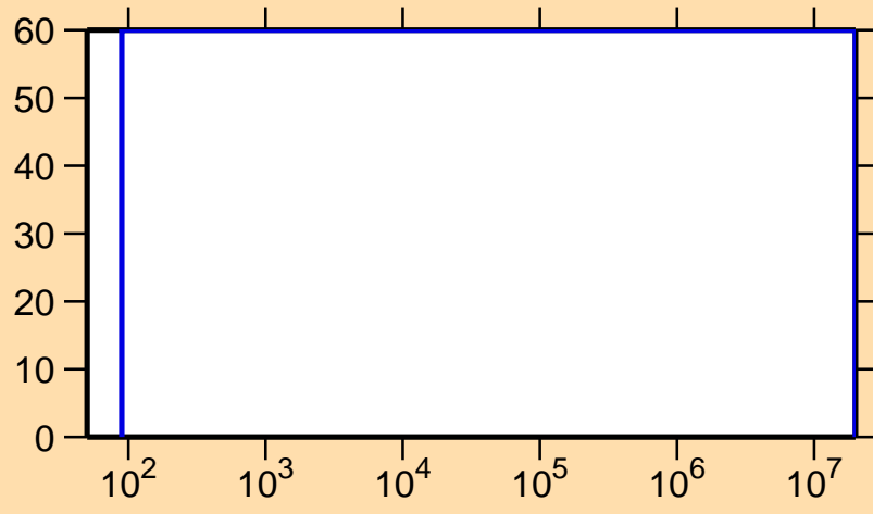
\Delta\sigma/\sigma vs. E for ^{227}\text{U}(n,p)
