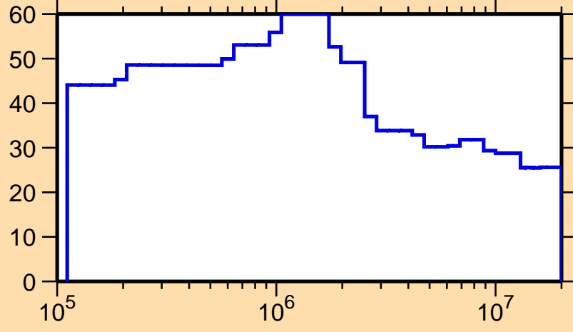
\Delta\sigma/\sigma vs. E for ^{227}\text{U}(n, nonel.)
