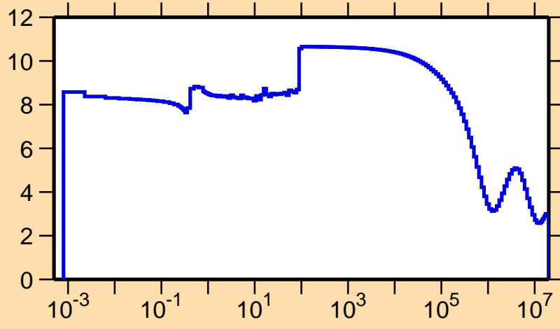
\sigma vs. E for ^{227}\text{U}(n,\text{el.})
