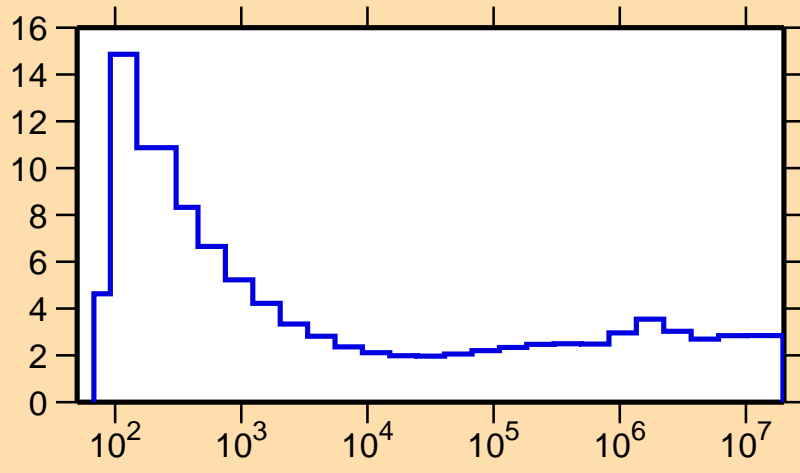
\sigma vs. E for ^{227}\text{U}(n,\text{nonel.})
