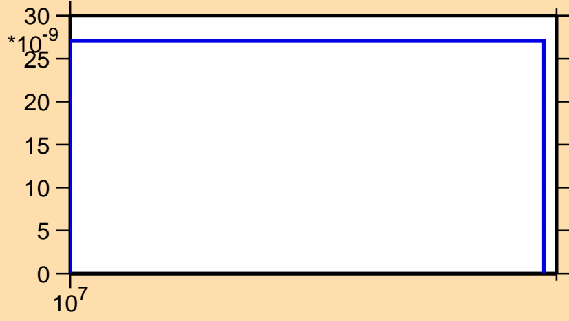
\sigma vs. E for ^{227}\text{U}(n,nd)
