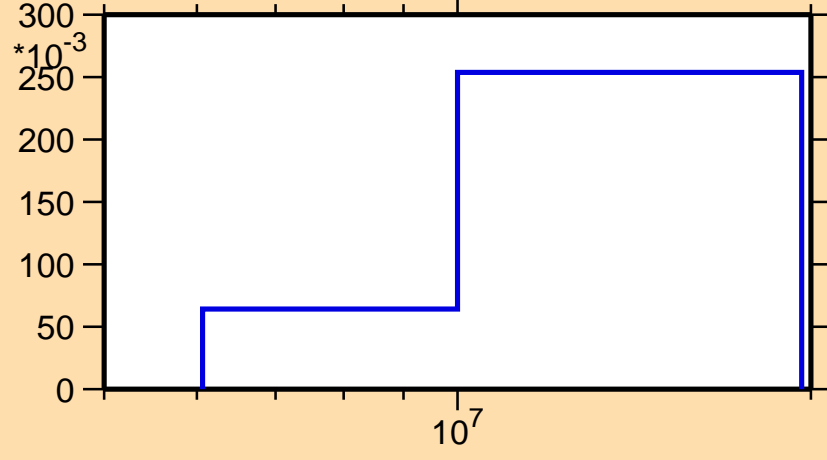
\sigma vs. E for ^{227}\text{U}(n,2n)
