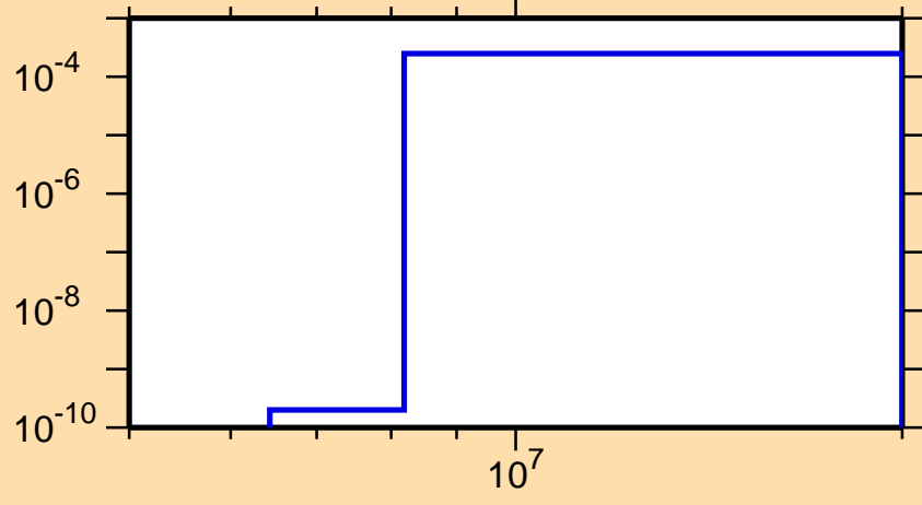
\sigma vs. E for ^{227}\text{U}(n,np)
