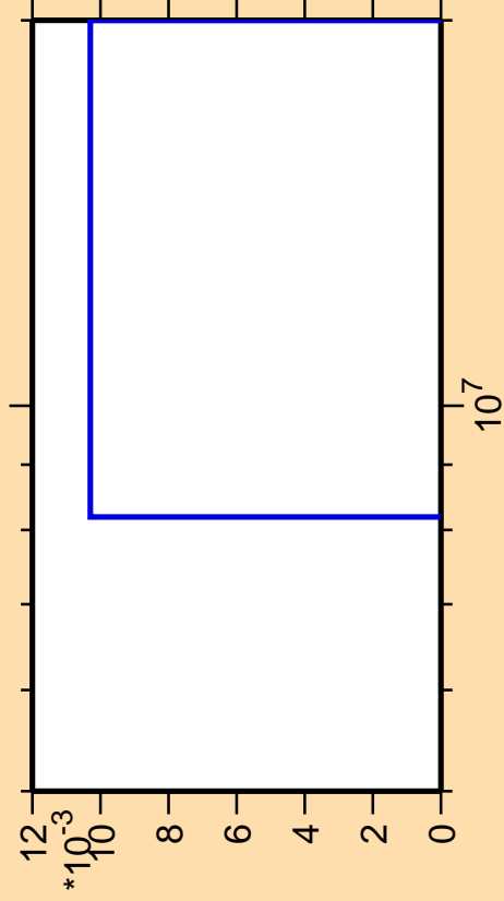
\Delta\sigma/\sigma vs. E for ^{227}\text{U}(n,\text{pt})
