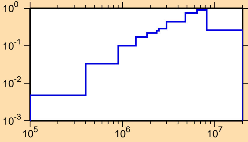
\sigma vs. E for ^{227}\text{U}(n,n\alpha)
