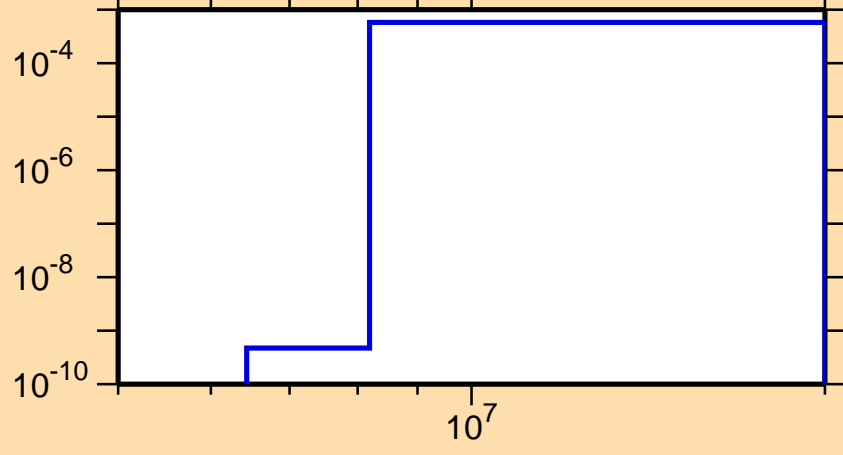
\sigma vs. E for ^{227}\text{U}(n,d)
