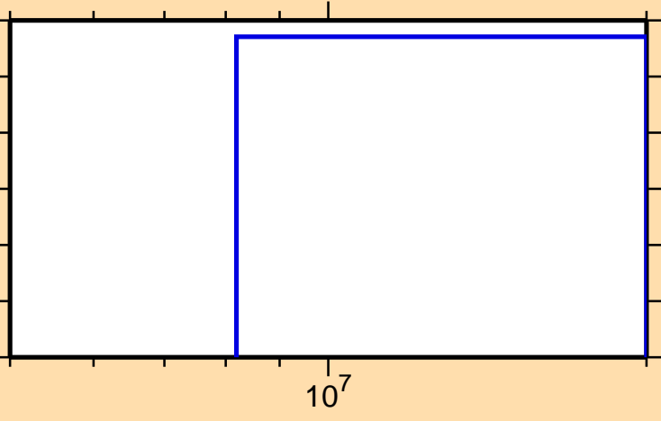
\sigma vs. E for ^{227}\text{U}(n,3n\alpha)
