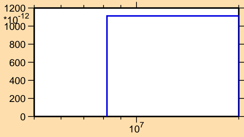
\sigma vs. E for ^{227}\text{U}(n,\text{He3})
