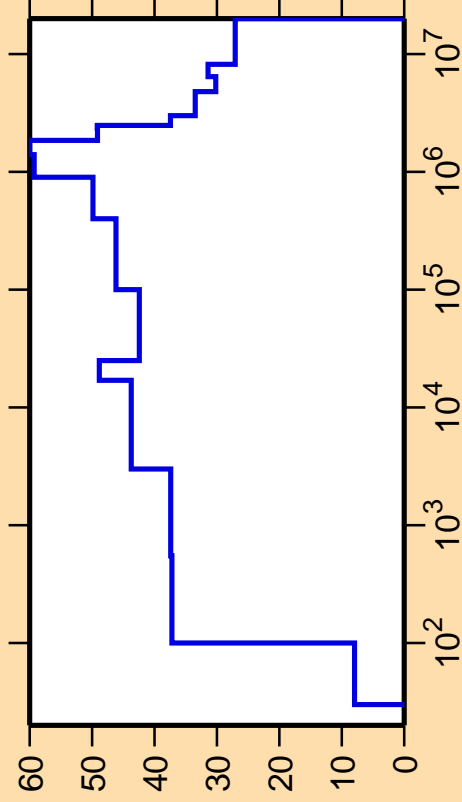
\Delta\sigma/\sigma vs. E for ^{227}\text{U}(n,\text{nonel.})
