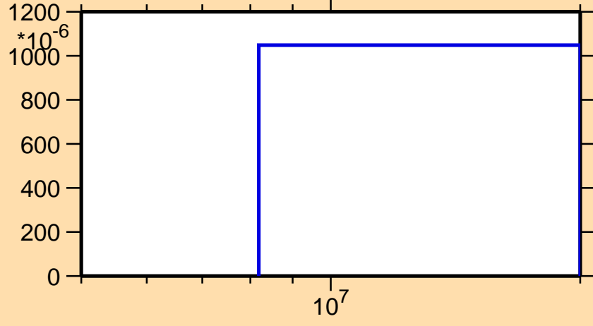
\sigma vs. E for ^{227}\text{U}(n,3n)
