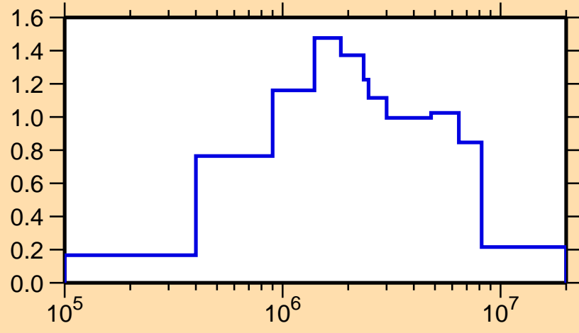
\sigma vs. E for ^{227}\text{U}(n,\text{inel.})
