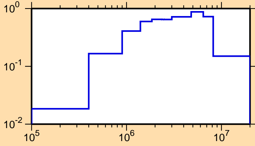
\sigma vs. E for ^{227}\text{U}(n,n\text{cont.})
