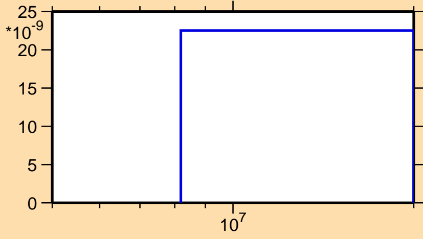
\sigma vs. E for ^{227}\text{U}(n,\text{nd})
