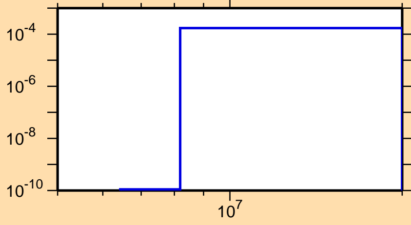
\sigma vs. E for ^{227}\text{U} (mt 45)
