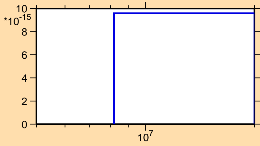
\sigma vs. E for ^{227}\text{U}(n,\text{pt})
