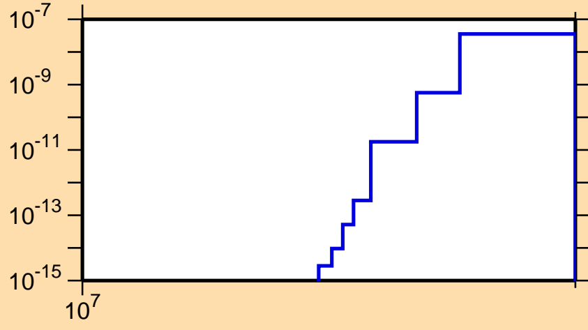
\sigma vs. E for ^{228}\text{U}(n,nt)
