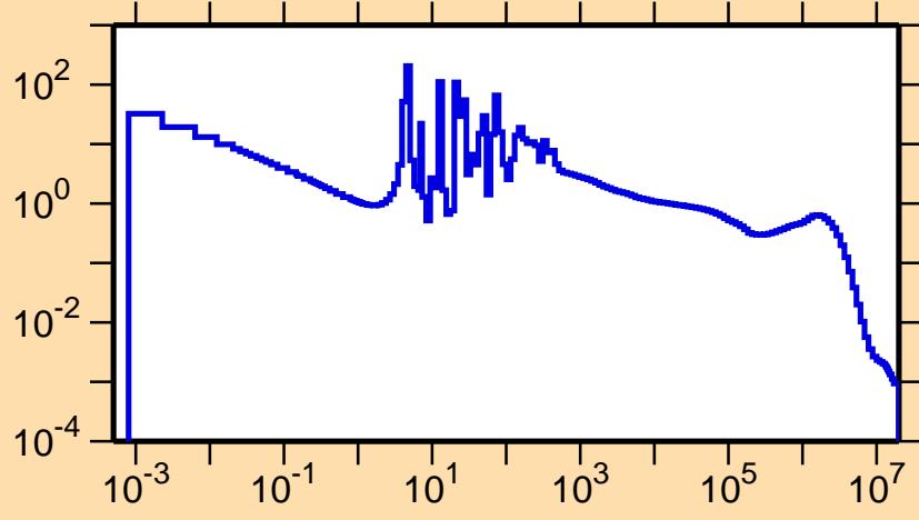
\sigma vs. E for ^{228}\text{U}(n,\gamma)
