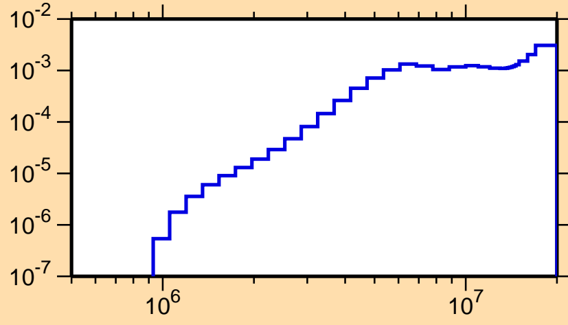
\sigma vs. E for ^{228}\text{U}(n,n\alpha)
