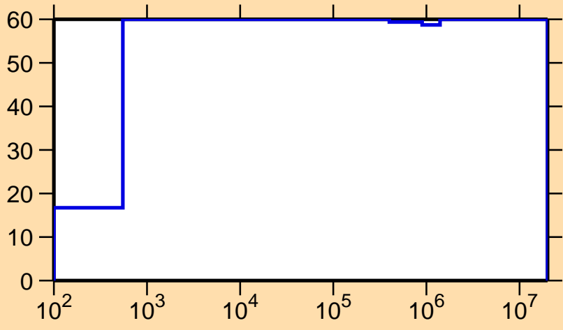
\Delta\sigma/\sigma vs. E for ^{228}\text{U}(n,\gamma)
