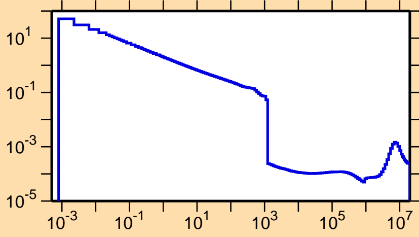
\sigma vs. E for ^{229}\text{U}(n,\gamma)
