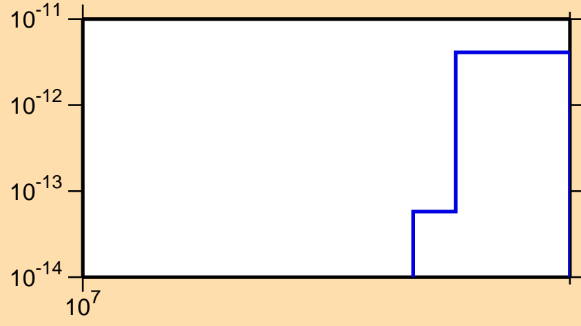
\sigma vs. E for ^{229}\text{U} (mt 34)
