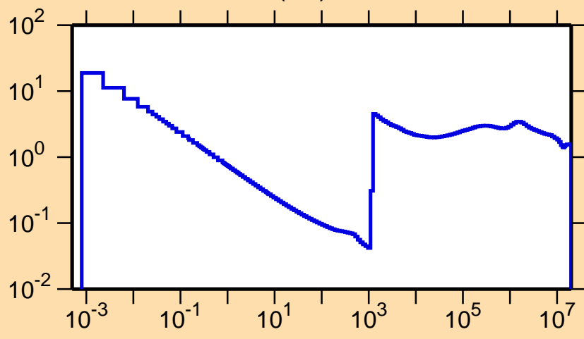
\sigma vs. E for ^{229}\text{U}(n,f)
