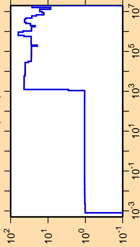
\Delta\sigma/\sigma vs. E for ^{229}\text{U}(n,\text{el.})
