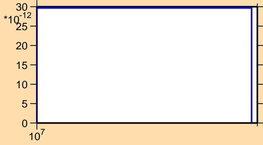
\sigma vs. E for ^{229}\text{U}(n,\text{nd})
