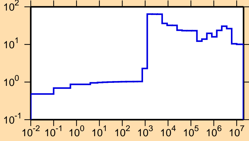
\Delta\sigma/\sigma vs. E for ^{229}\text{U}(n,tot.)
