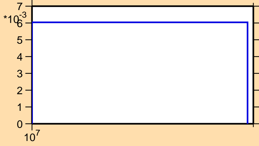
\sigma vs. E for ^{229}\text{U}(n,3n\alpha)
