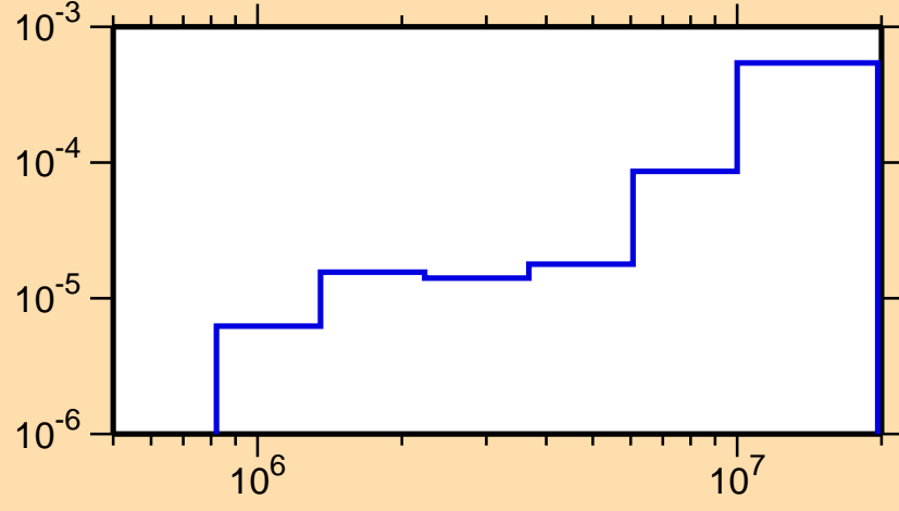
\sigma vs. E for ^{229}\text{U}(n,n\alpha)
