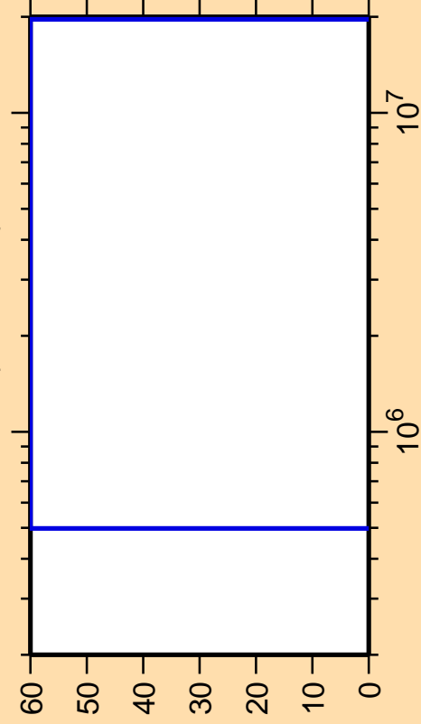
\Delta\sigma/\sigma vs. E for ^{229}\text{U}(n,\text{ncont.})
