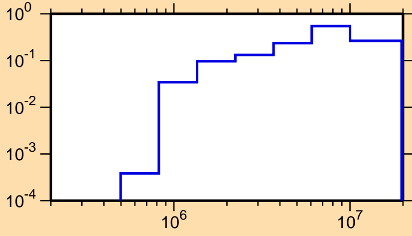
\sigma vs. E for ^{229}\text{U}(n,n\text{cont.})
