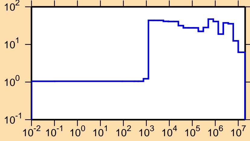
\Delta\sigma/\sigma vs. E for ^{229}\text{U}(n,el.)
