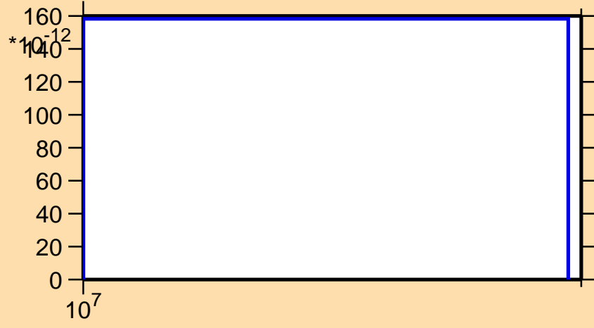
\sigma vs. E for ^{229}\text{U}(n,\text{He}3)
