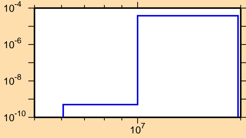
\sigma vs. E for ^{229}\text{U}(\text{mt117})
