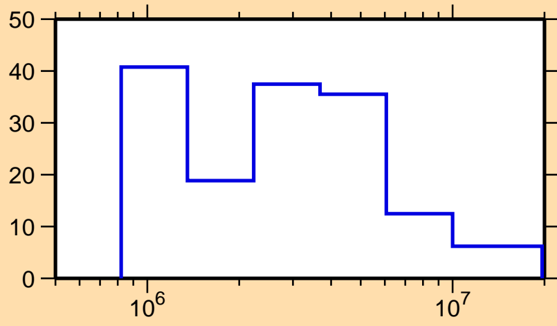
\Delta\sigma/\sigma vs. E for ^{229}\text{U}(n,el.)
