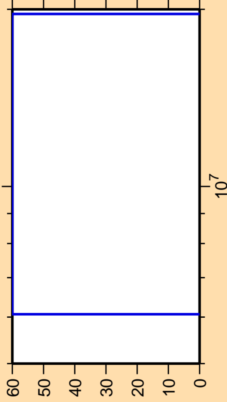
\Delta\sigma/\sigma vs. E for ^{229}\text{U} (mt 45)
