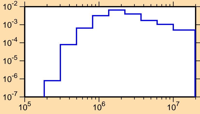
\sigma vs. E for ^{229}\text{U}(n,n_4)
