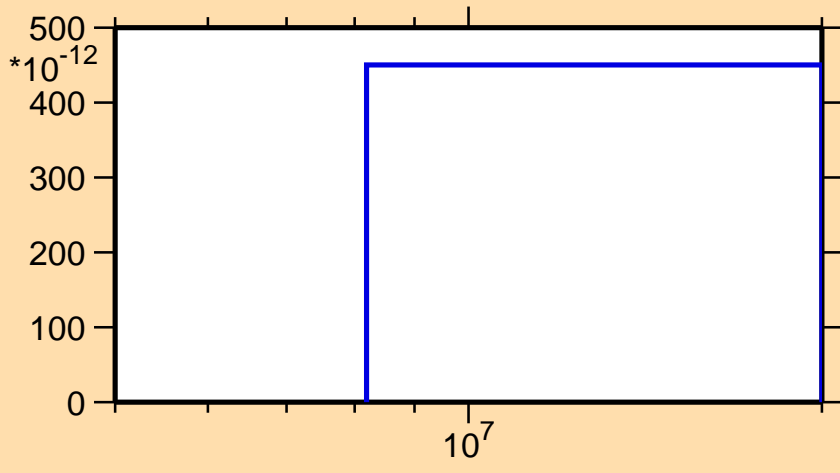
\sigma vs. E for ^{229}\text{U}(n,2np)
