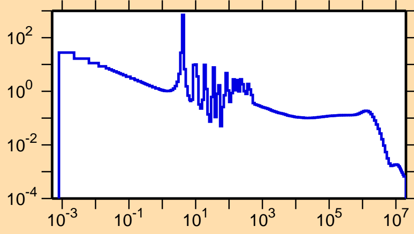
\sigma vs. E for ^{230}\text{U}(n,\gamma)
