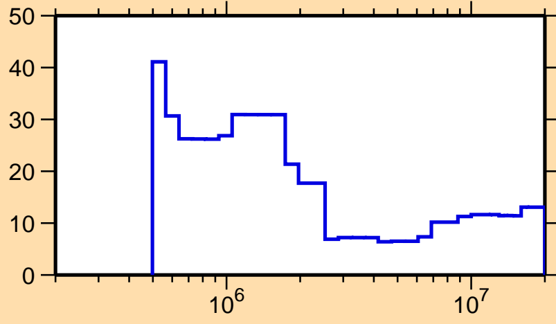
\Delta\sigma/\sigma vs. E for ^{230}\text{U}(n, nonel.)
