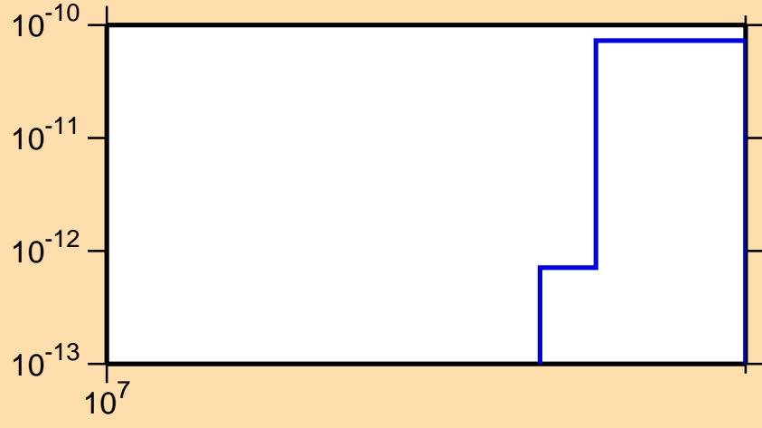
\sigma vs. E for ^{230}\text{U}(n,nt)
