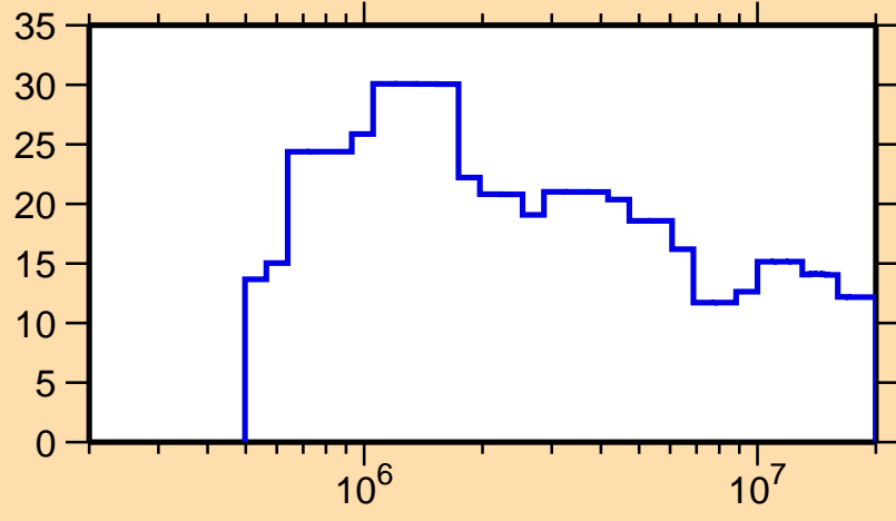
\Delta\sigma/\sigma vs. E for ^{230}\text{U}(n, el.)
