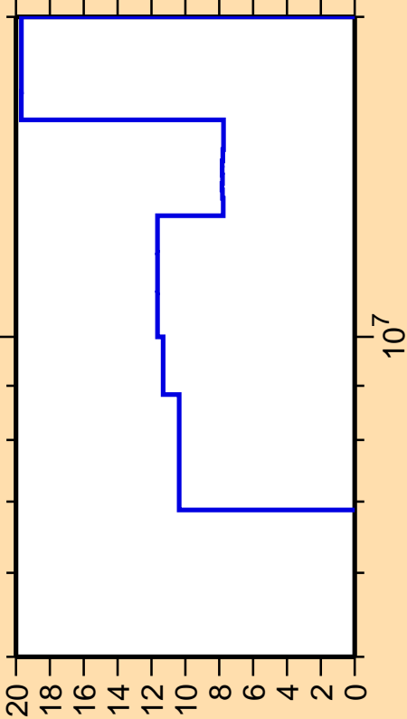
\Delta\sigma/\sigma vs. E for ^{230}\text{U}(n,f)
