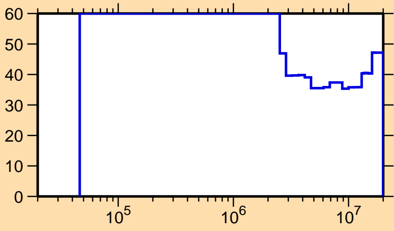
\Delta\sigma/\sigma vs. E for ^{230}\text{U}(n,n_1)
