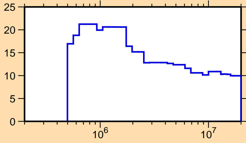
\Delta\sigma/\sigma vs. E for ^{230}\text{U}(n, tot.)
