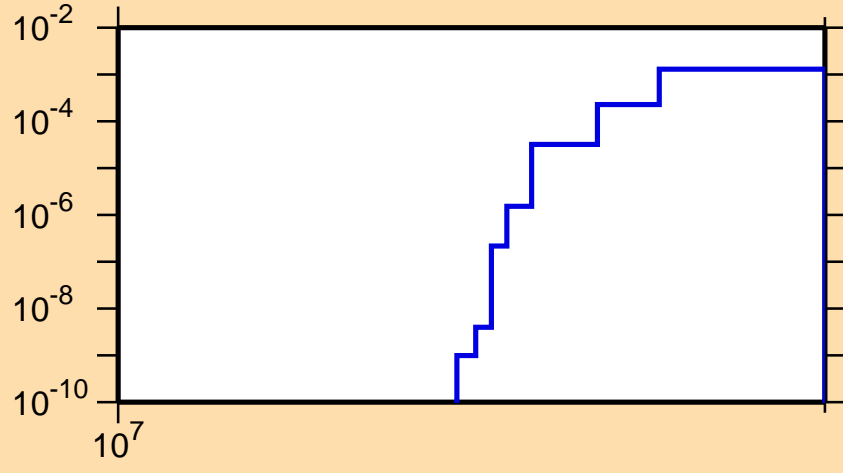
\sigma vs. E for ^{230}\text{U}(n,3n\alpha)
