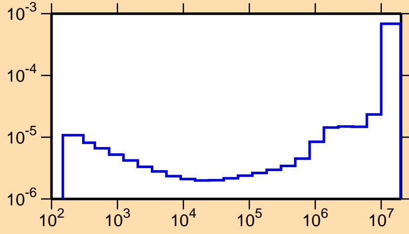
\sigma vs. E for ^{230}\text{U}(n,\alpha)
