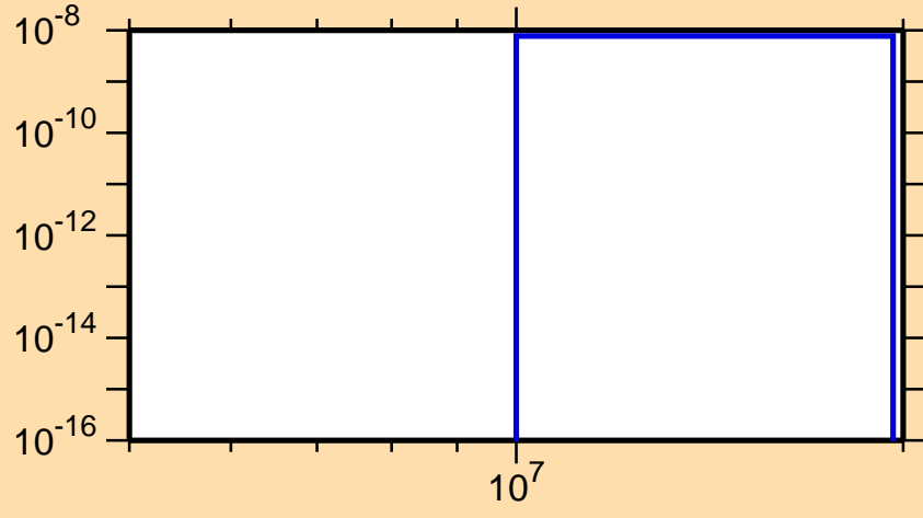
\sigma vs. E for ^{230}\text{U}(\text{mt117})
