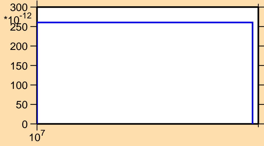
\sigma vs. E for ^{230}\text{U}(n,nd)
