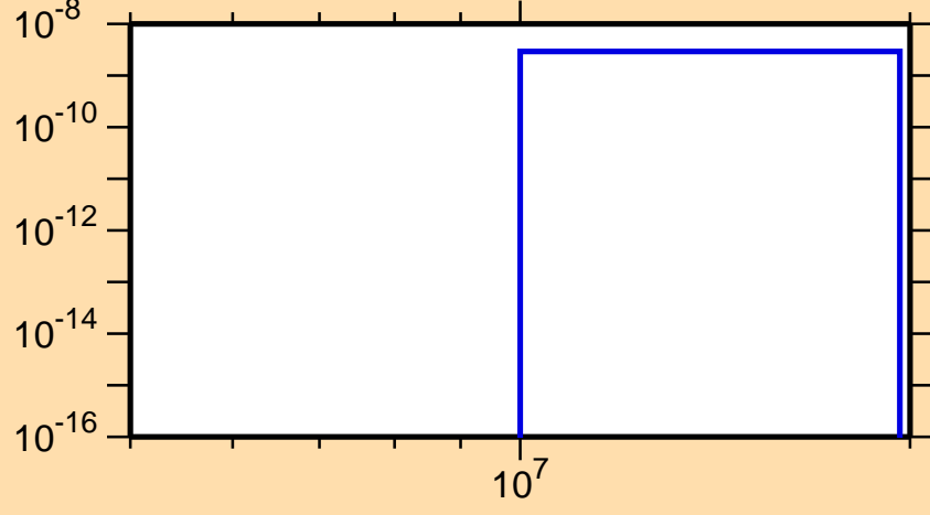
\sigma vs. E for ^{230}\text{U} (mt 45)
