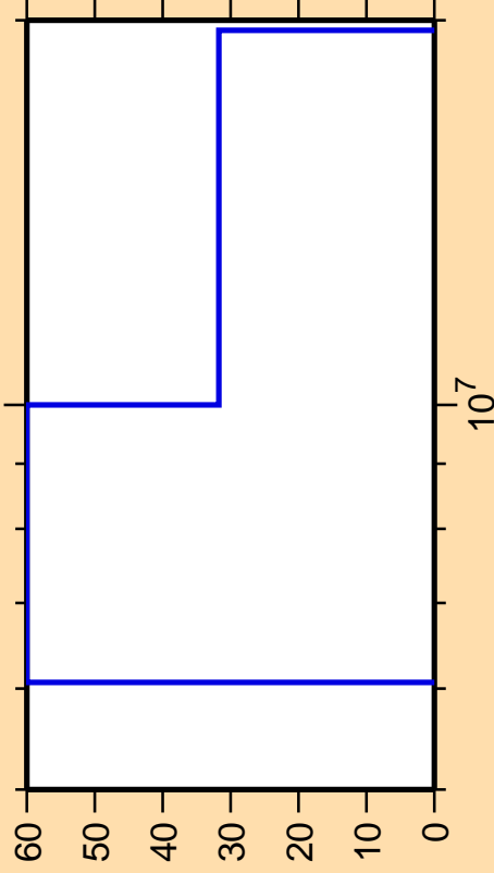
\Delta\sigma/\sigma vs. E for ^{230}\text{U}(n,d)
