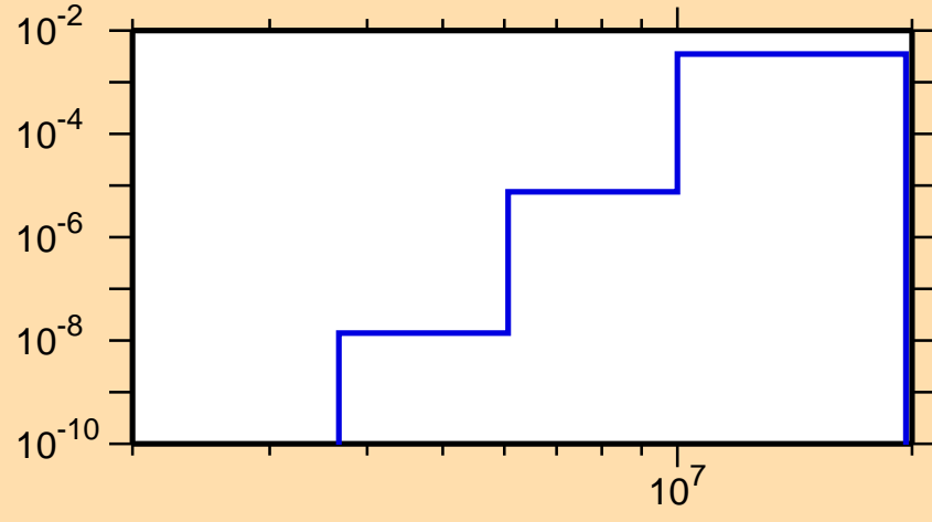
\sigma vs. E for ^{230}\text{U}(n,p)
