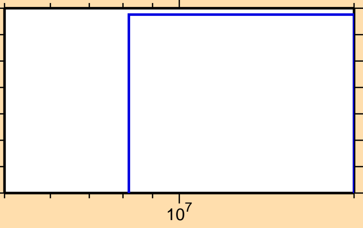
\sigma vs. E for ^{230}\text{U}(n,3n)
