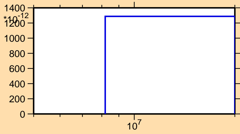
\sigma vs. E for ^{230}\text{U}(n,p\alpha)
