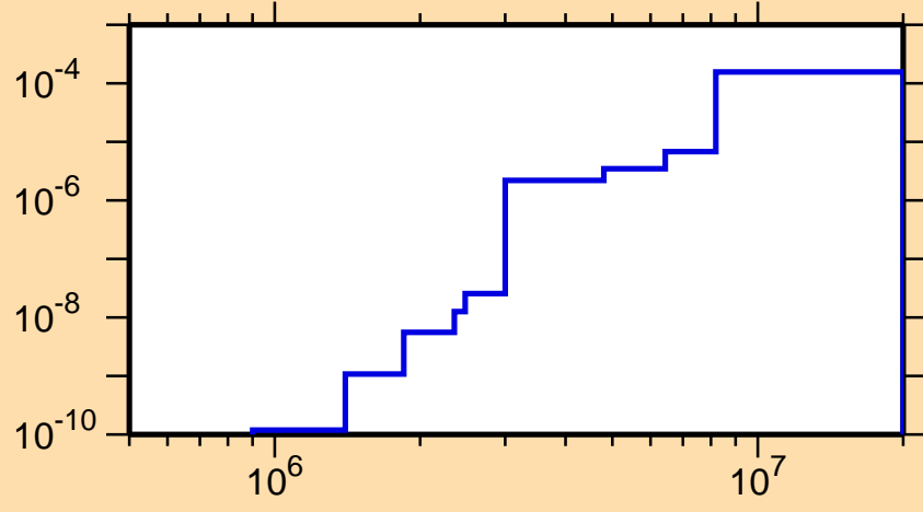
\sigma vs. E for ^{230}\text{U}(n,n\alpha)
