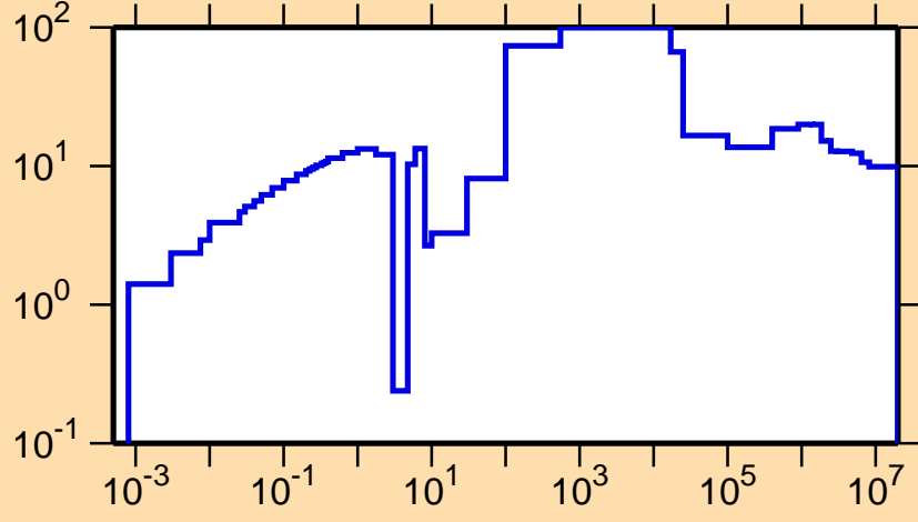
\Delta\sigma/\sigma vs. E for ^{230}\text{U}(n,tot.)
