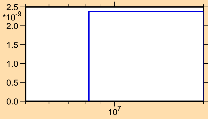
\sigma vs. E for ^{230}\text{U} (mt 45)
