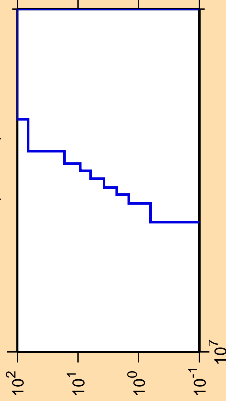
\Delta\sigma/\sigma vs. E for ^{231}\text{U} (mt117)
