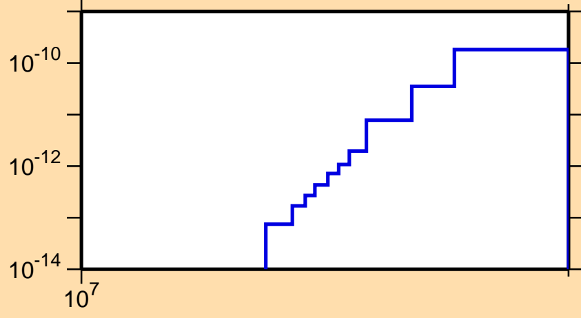
\sigma vs. E for ^{231}\text{U} (mt117)
