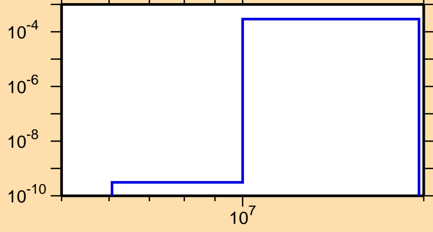
\sigma vs. E for ^{231}\text{U}(n,d)
