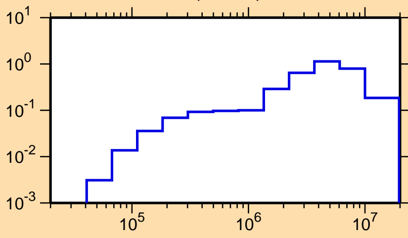
\sigma vs. E for ^{231}\text{U}(n,\text{inel.})
