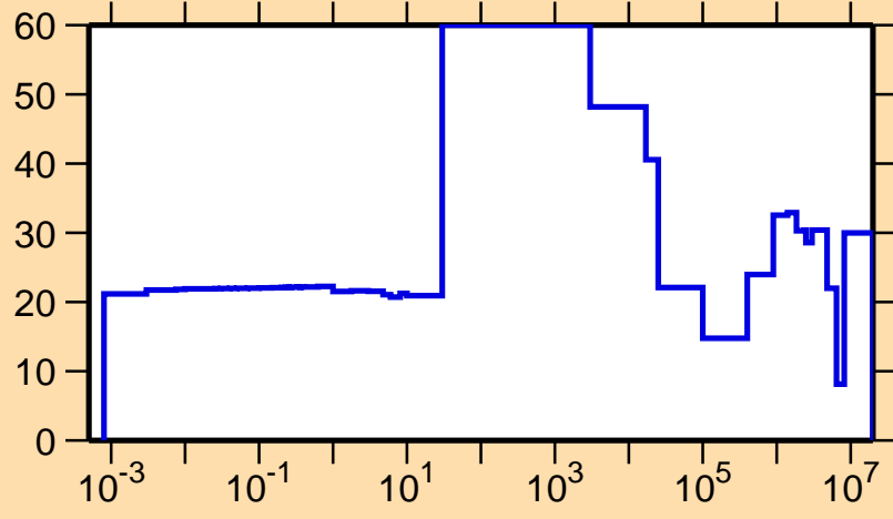
\Delta\sigma/\sigma vs. E for ^{231}\text{U}(n,el.)
