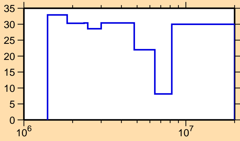
\Delta\sigma/\sigma vs. E for ^{231}\text{U}(n,el.)
