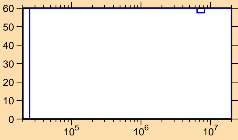
\Delta\sigma/\sigma vs. E for ^{231}\text{U}(n,n_1)
