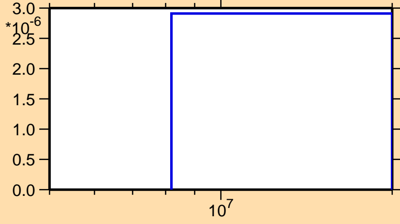
\sigma vs. E for ^{231}\text{U}(n,3n\alpha)
