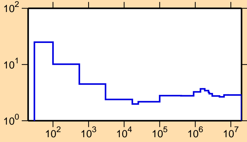
\sigma vs. E for ^{231}\text{U}(n,\text{nonel.})
