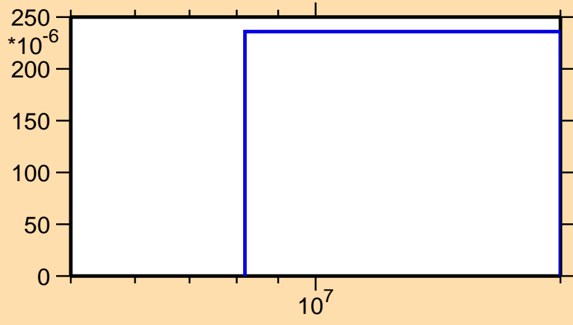
\sigma vs. E for ^{231}\text{U}(n,3n)
