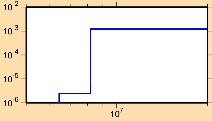
\sigma vs. E for ^{231}\text{U}(n,2n\alpha)
