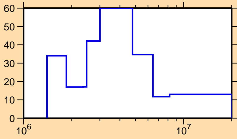
\Delta\sigma/\sigma vs. E for ^{231}\text{U}(n,f)
