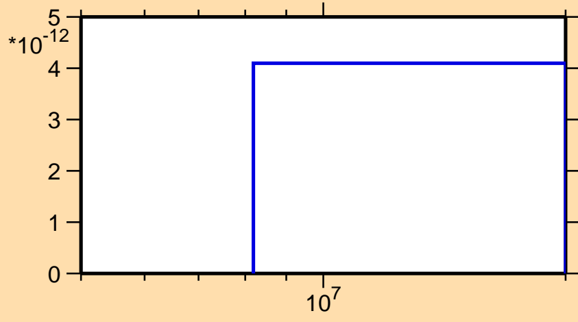
\sigma vs. E for ^{231}\text{U}(\text{mt117})
