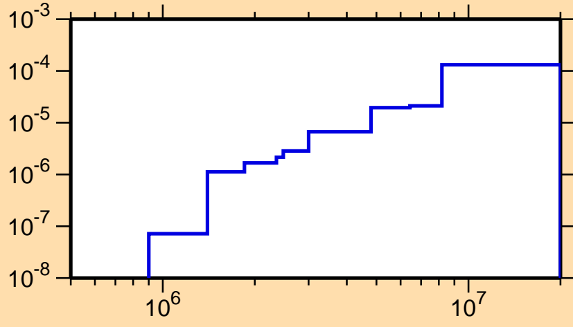
\sigma vs. E for ^{231}\text{U}(n,n\alpha)
