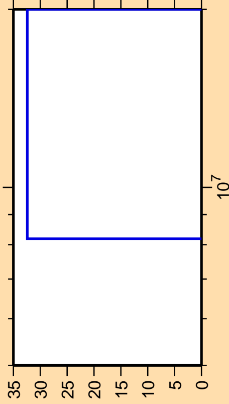
\Delta\sigma/\sigma vs. E for ^{231}\text{U}(\text{mt117})
