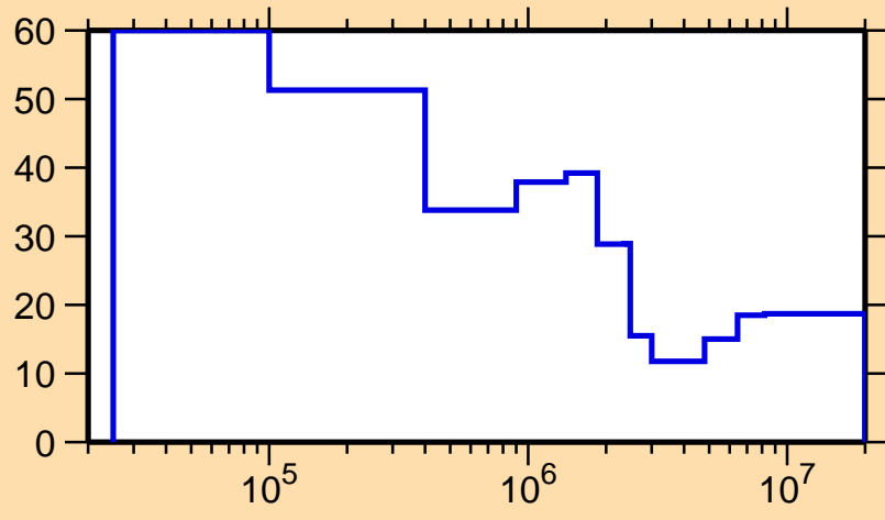
\Delta\sigma/\sigma vs. E for ^{231}\text{U}(n,\text{nonel.})
