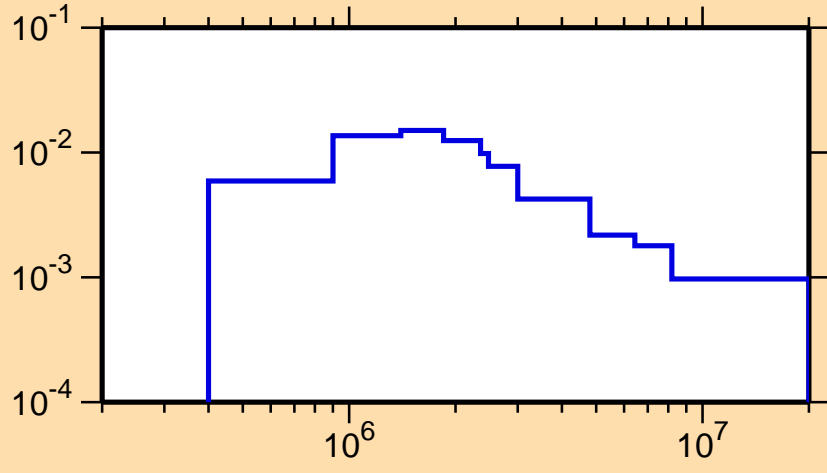
\sigma vs. E for ^{231}\text{U}(n,n_3)
