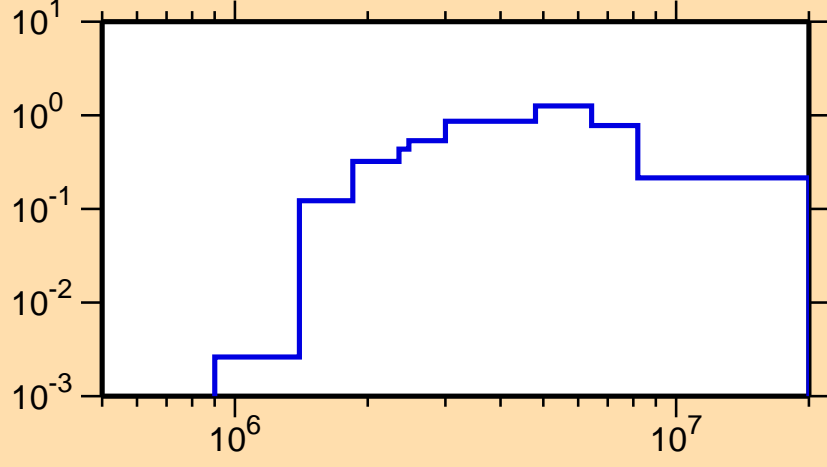
\sigma vs. E for ^{231}\text{U}(n,n\text{cont.})
