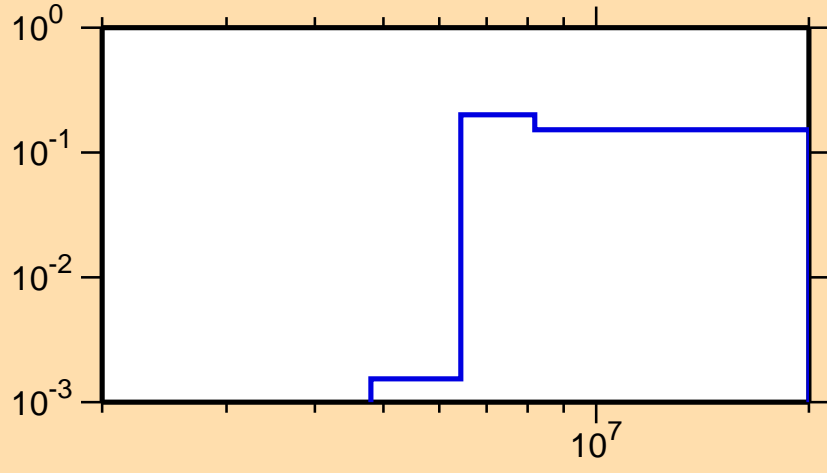
\sigma vs. E for ^{231}\text{U}(n,2n)
