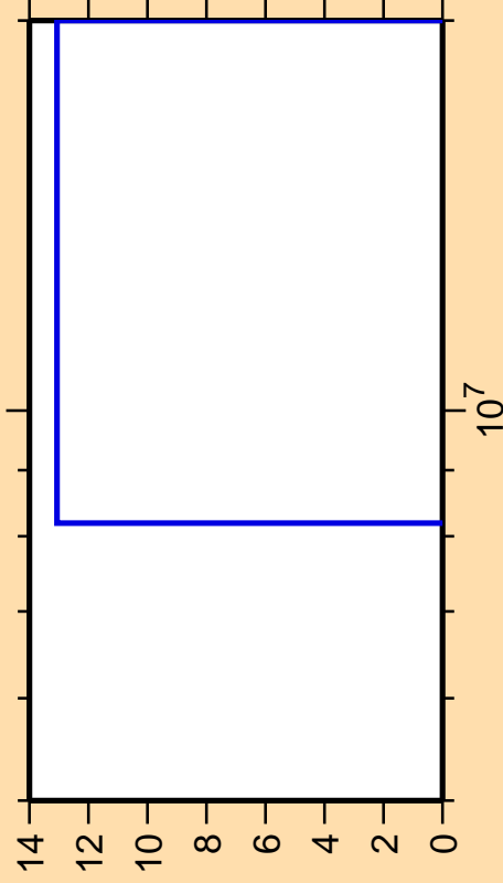
\Delta\sigma/\sigma vs. E for ^{231}\text{U} (mt 45)
