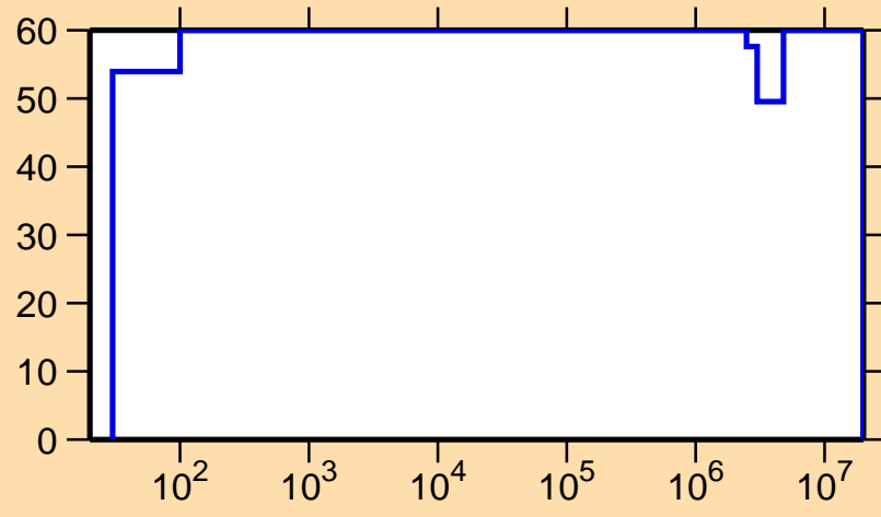
\Delta\sigma/\sigma vs. E for ^{231}\text{U}(n,\gamma)
