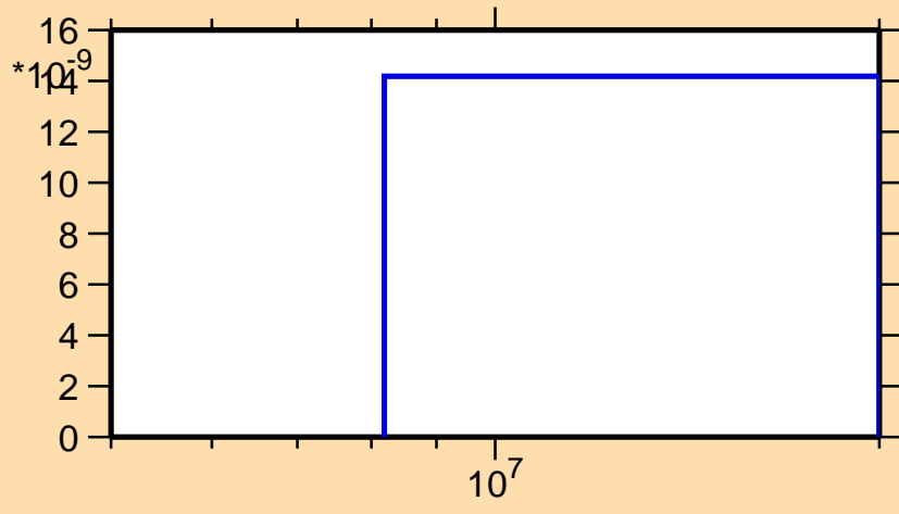
\sigma vs. E for ^{231}\text{U}(n,\text{nd})
