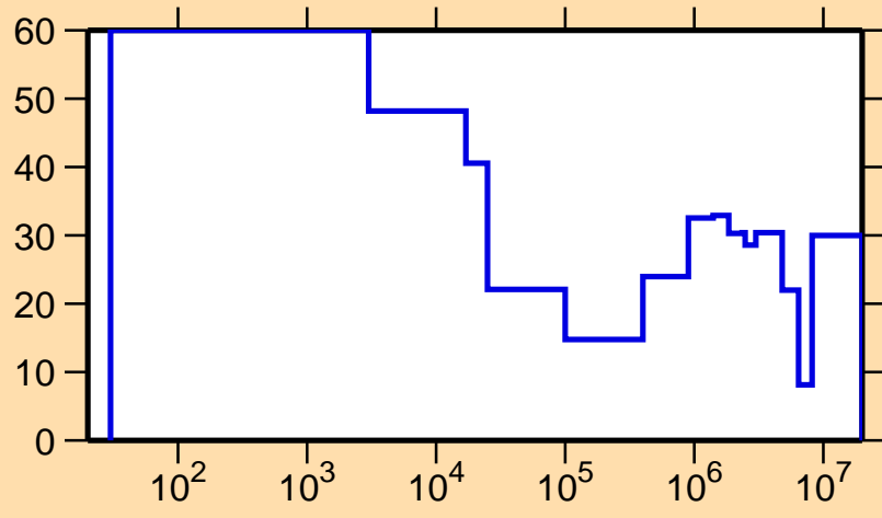
\Delta\sigma/\sigma vs. E for ^{231}\text{U}(n,\text{el.})
