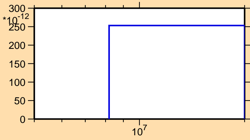
\sigma vs. E for ^{231}\text{U}(n,nt)
