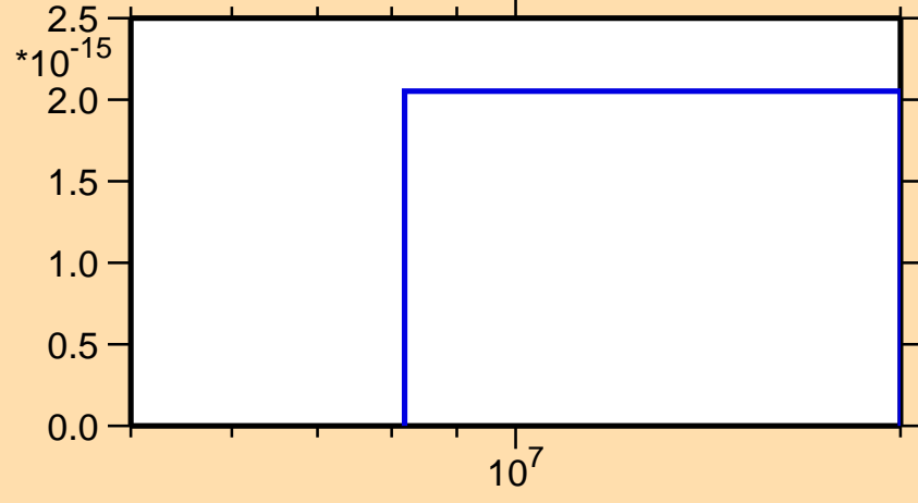
\sigma vs. E for ^{231}\text{U} (mt 34)
