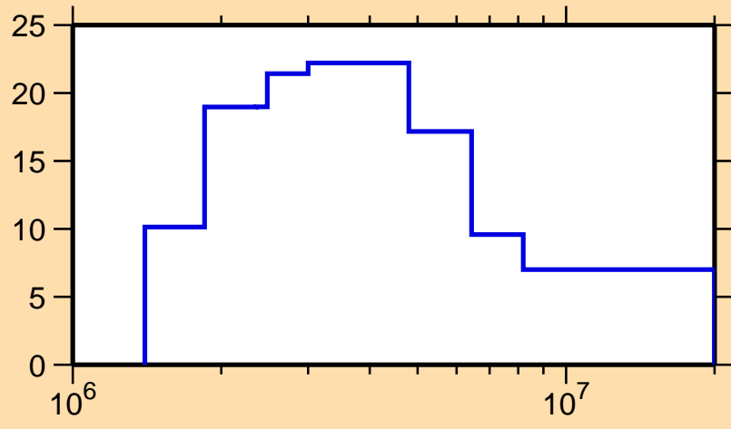
\Delta\sigma/\sigma vs. E for ^{231}\text{U}(n,\text{tot.})
