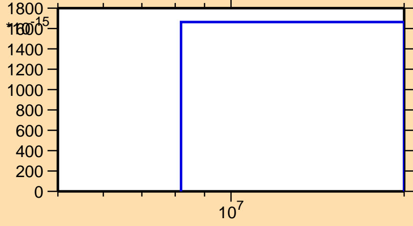
\sigma vs. E for ^{231}\text{U} (mt 45)
