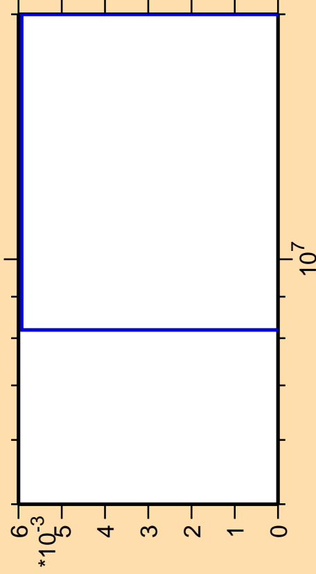
\Delta\sigma/\sigma vs. E for ^{231}\text{U} (mt 34)
