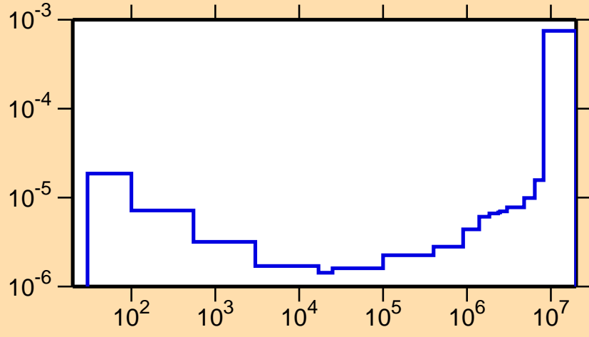
\sigma vs. E for ^{231}\text{U}(n,\alpha)
