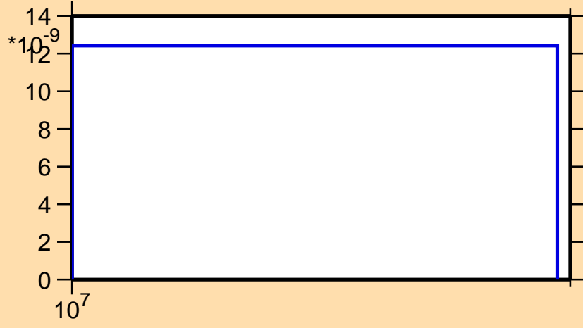
\sigma vs. E for ^{233}\text{U}(n,nd)
