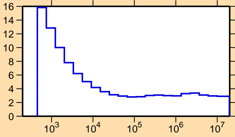
\sigma vs. E for ^{233}\text{U}(n,\text{nonel.})
