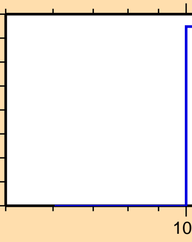
\sigma vs. E for ^{233}\text{U}(n,t)
