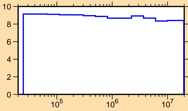
\Delta\sigma/\sigma vs. E for ^{233}\text{U}(n,inel.)
