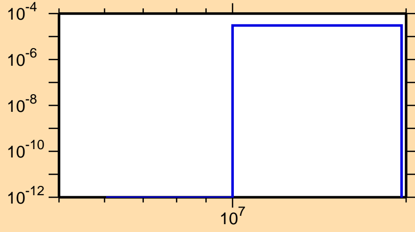
\sigma vs. E for ^{233}\text{U}(n,t)
