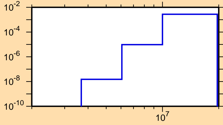
\sigma vs. E for ^{233}\text{U}(n,p)
