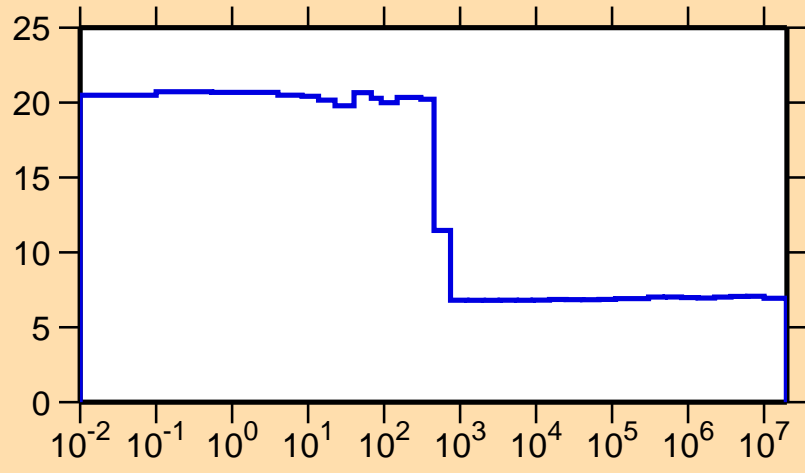
\Delta\sigma/\sigma vs. E for ^{233}\text{U}(n,el.)
