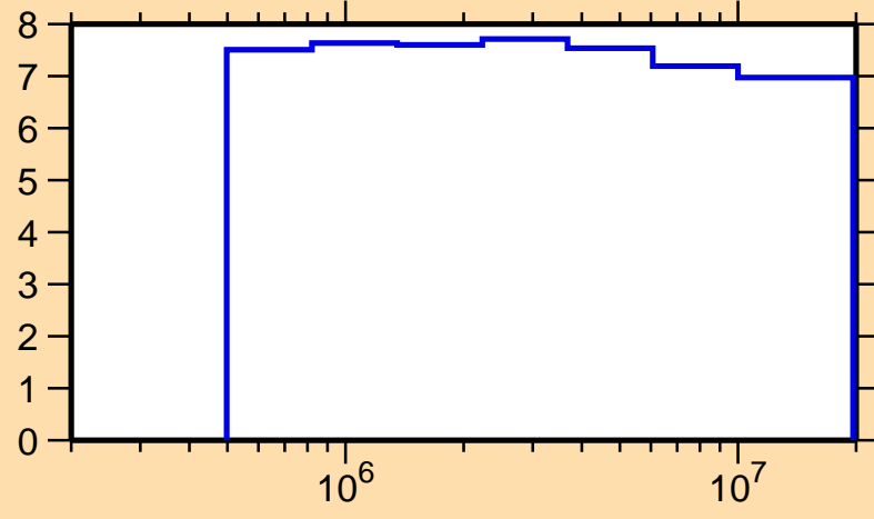
\Delta\sigma/\sigma vs. E for ^{233}\text{U}(n,n\text{cont.})
