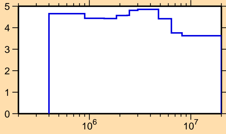
\Delta\sigma/\sigma vs. E for ^{233}\text{U}(n,tot.)
