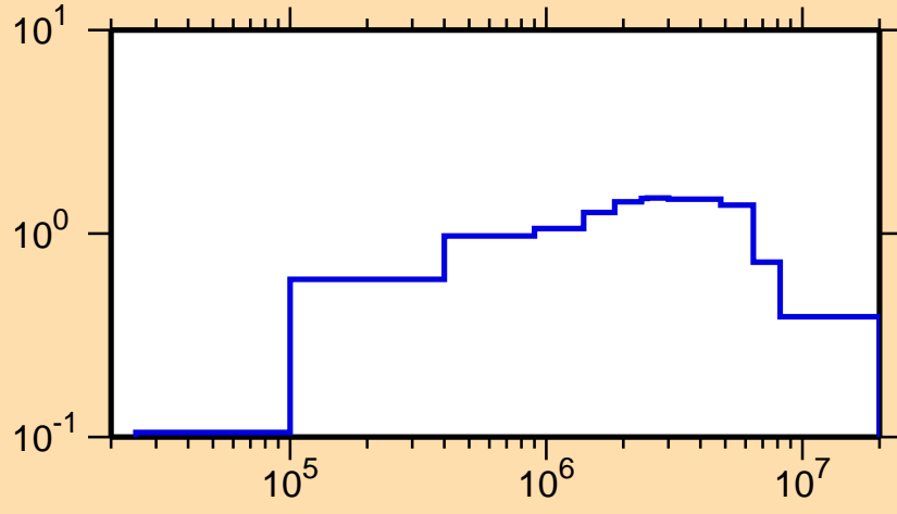
\sigma vs. E for ^{233}\text{U}(n,\text{inel.})
