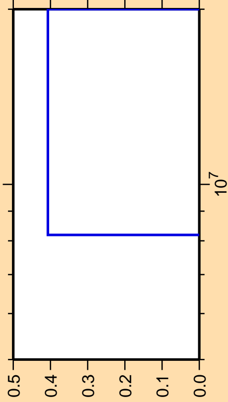
\Delta\sigma/\sigma vs. E for ^{233}\text{U}(n,t)
