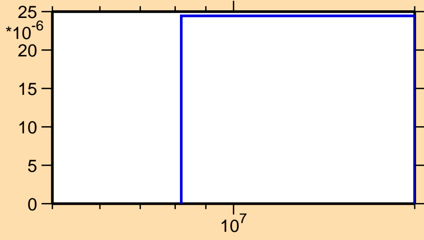
\sigma vs. E for ^{233}\text{U}(n,t)
