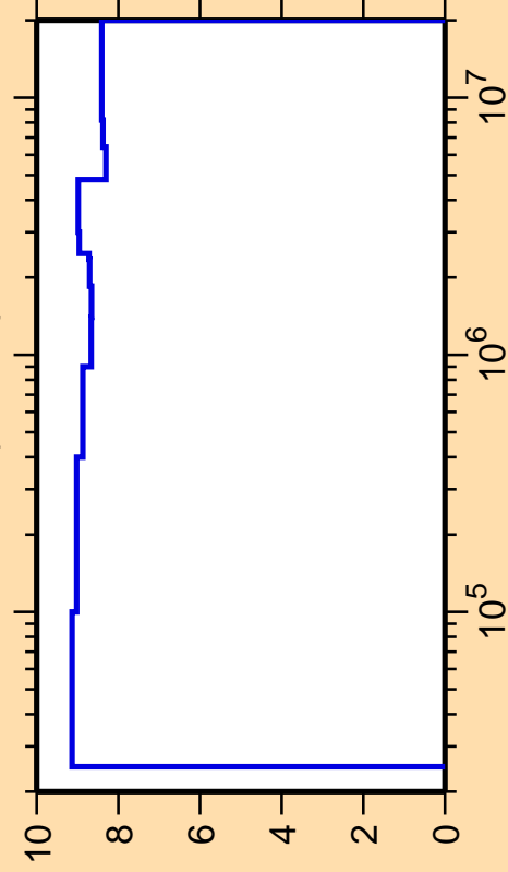
\Delta\sigma/\sigma vs. E for ^{233}\text{U}(n,\text{inel.})
