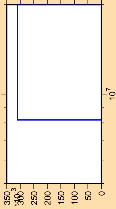
\Delta\sigma/\sigma vs. E for ^{233}\text{U}(n,d)
