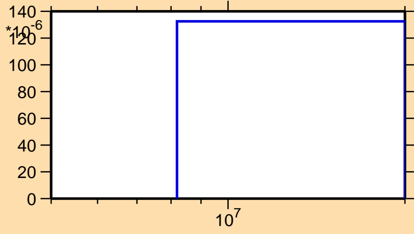
\sigma vs. E for ^{233}\text{U}(n,d)
