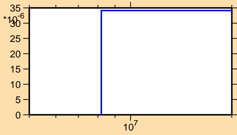
\sigma vs. E for ^{233}\text{U}(n,3n\alpha)
