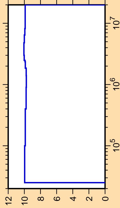
\Delta\sigma/\sigma vs. E for ^{233}\text{U}(n,n_2)
