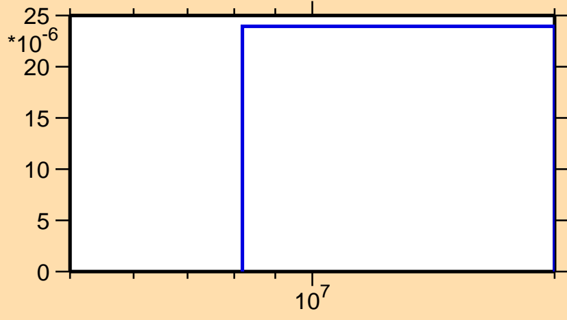
\sigma vs. E for ^{233}\text{U}(n,np)
