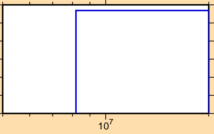
\sigma vs. E for ^{233}\text{U}(n,2np)
