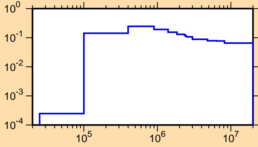
\sigma vs. E for ^{233}\text{U}(n,n_2)
