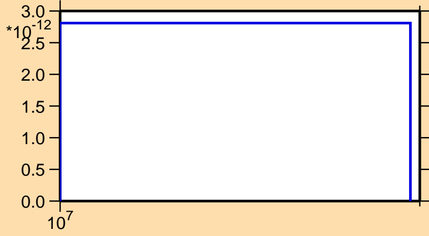
\sigma vs. E for ^{234}\text{U}(n,p\alpha)
