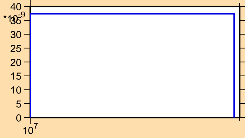
\sigma vs. E for ^{234}\text{U}(n,3n\alpha)
