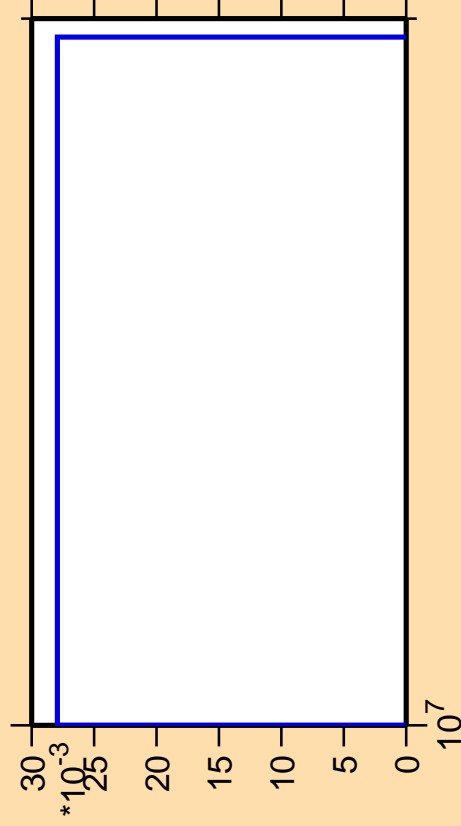
\Delta\sigma/\sigma vs. E for ^{234}\text{U} (mt117)
