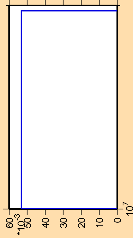
\Delta\sigma/\sigma vs. E for ^{234}\text{U}(n,p\alpha)
