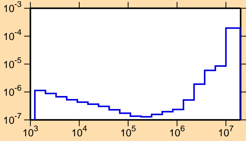
\sigma vs. E for ^{234}\text{U}(n,\alpha)
