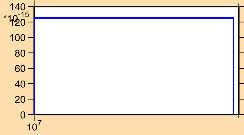
\sigma vs. E for ^{234}\text{U} (mt 45)
