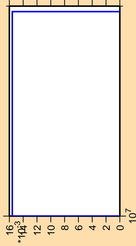
\Delta\sigma/\sigma vs. E for ^{234}\text{U} (mt 45)
