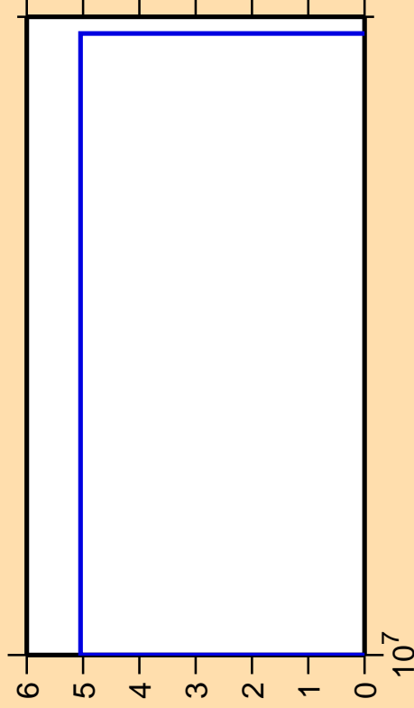
\Delta\sigma/\sigma vs. E for ^{234}\text{U}(n,nd)
