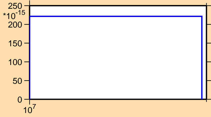
\sigma vs. E for ^{234}\text{U} (mt117)
