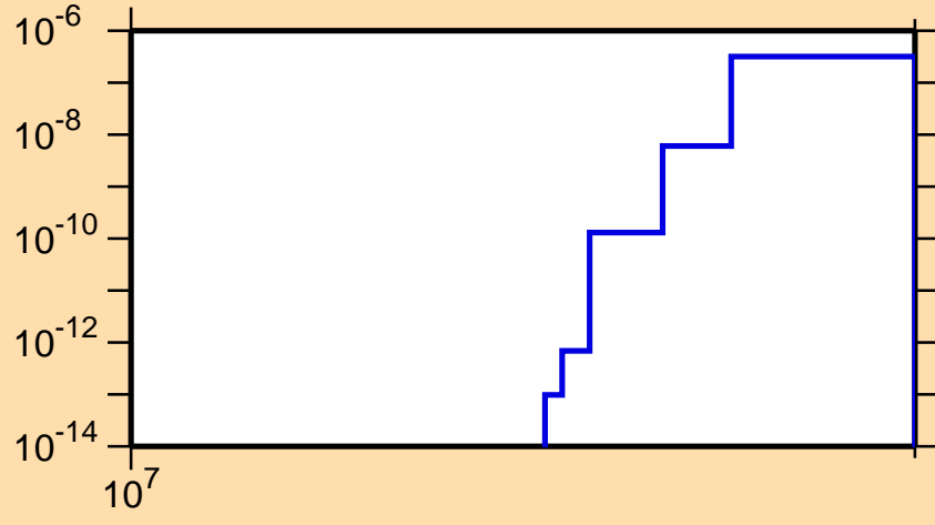
\sigma vs. E for ^{235}\text{U}(n,2np)
