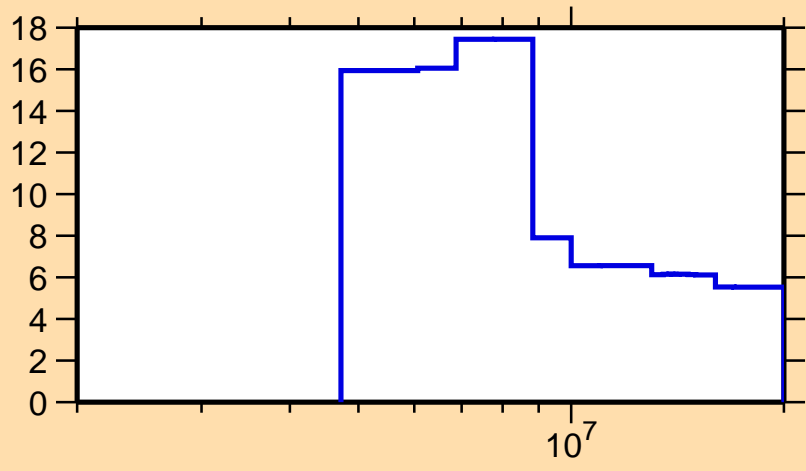
\Delta\sigma/\sigma vs. E for ^{235}\text{U}(n,\text{el.})
