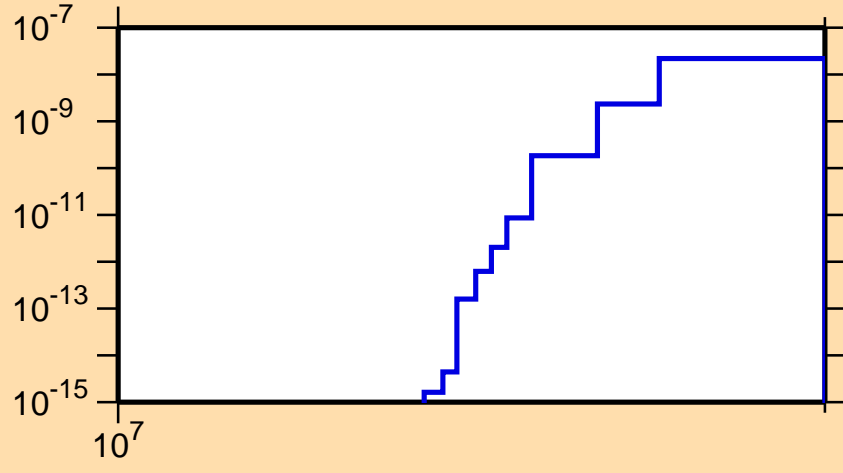
\sigma vs. E for ^{235}\text{U}(n,3n\alpha)
