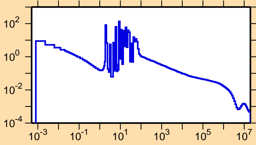
\sigma vs. E for ^{235}\text{U}(n,\gamma)
