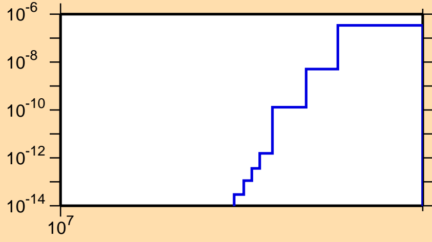
\sigma vs. E for ^{235}\text{U}(n,nt)
