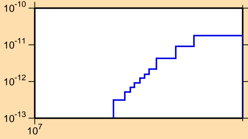
\sigma vs. E for ^{235}\text{U}(n,p\alpha)
