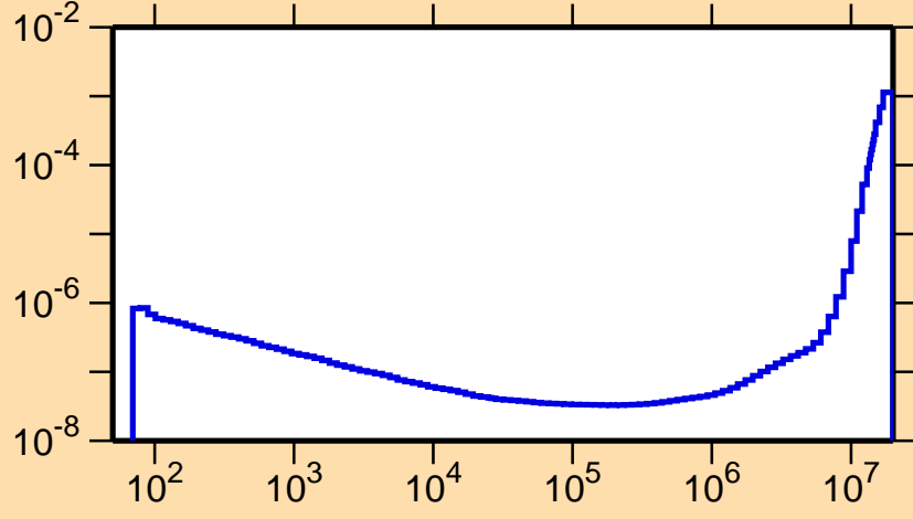
\sigma vs. E for ^{235}\text{U}(n,\alpha)
