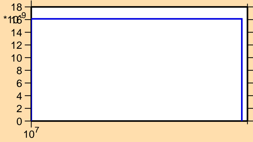
\sigma vs. E for ^{235}\text{U}(n,\text{nd})
