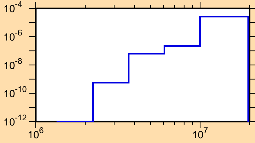
\sigma vs. E for ^{235}\text{U}(n,n\alpha)
