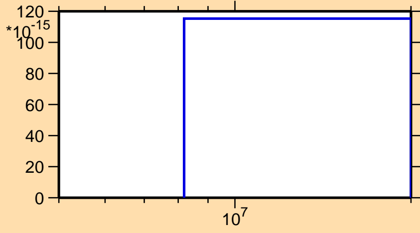
\sigma vs. E for ^{235}\text{U}(n,\text{He}3)
