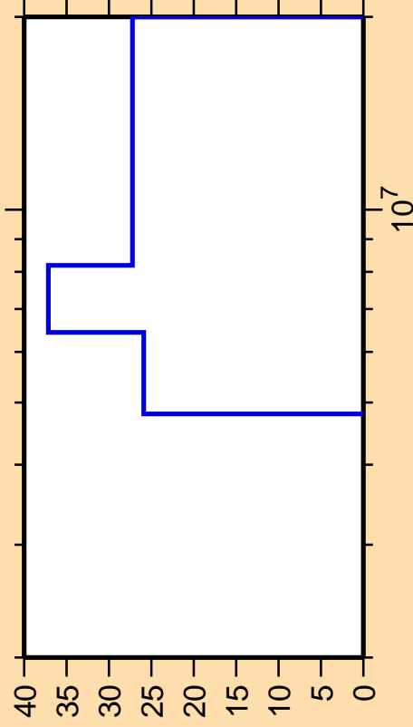
\Delta\sigma/\sigma vs. E for ^{235}\text{U}(n,n\text{cont.})
