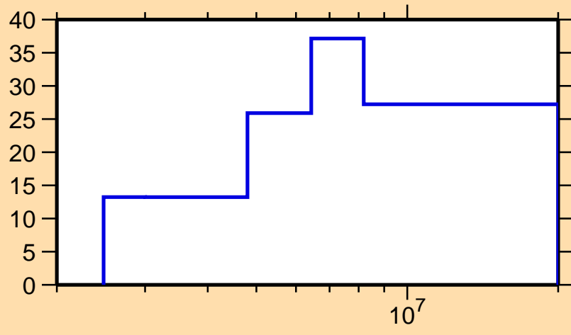
\Delta\sigma/\sigma vs. E for ^{235}\text{U}(n,ncont.)
