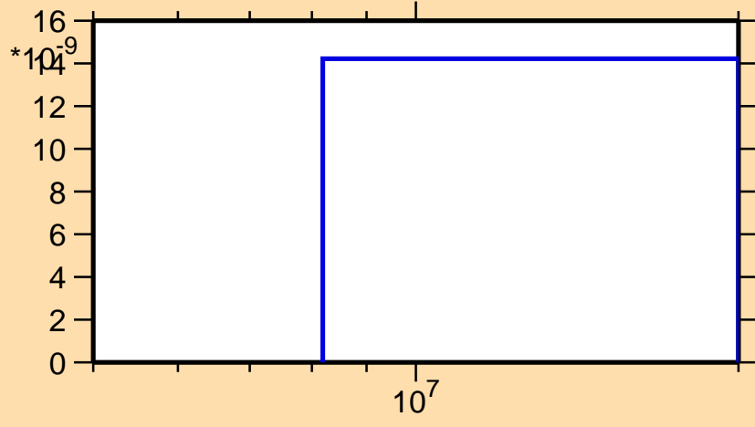
\sigma vs. E for ^{235}\text{U}(n,nd)
