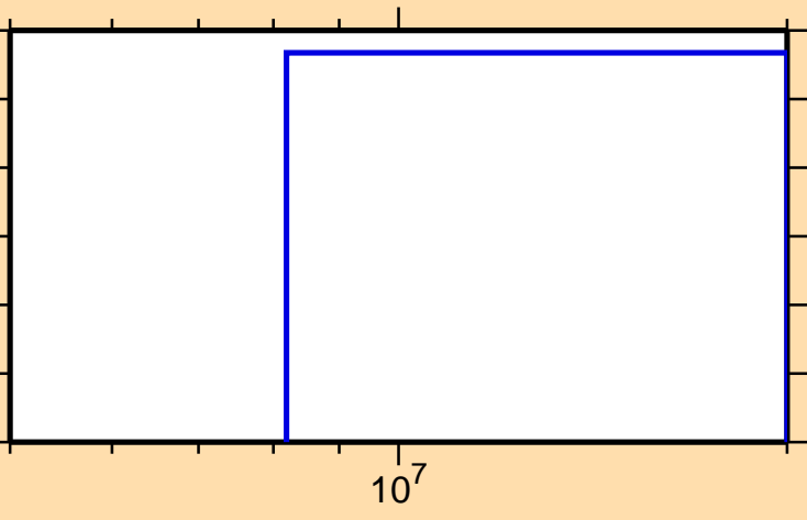
\sigma vs. E for ^{235}\text{U}(n,2np)
