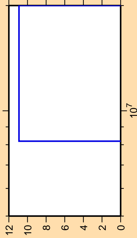
\Delta\sigma/\sigma vs. E for ^{235}\text{U}(n,p\alpha)
