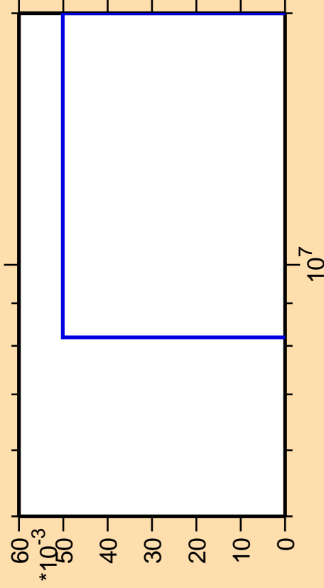
\Delta\sigma/\sigma vs. E for ^{235}\text{U}(n,\text{He}3)
