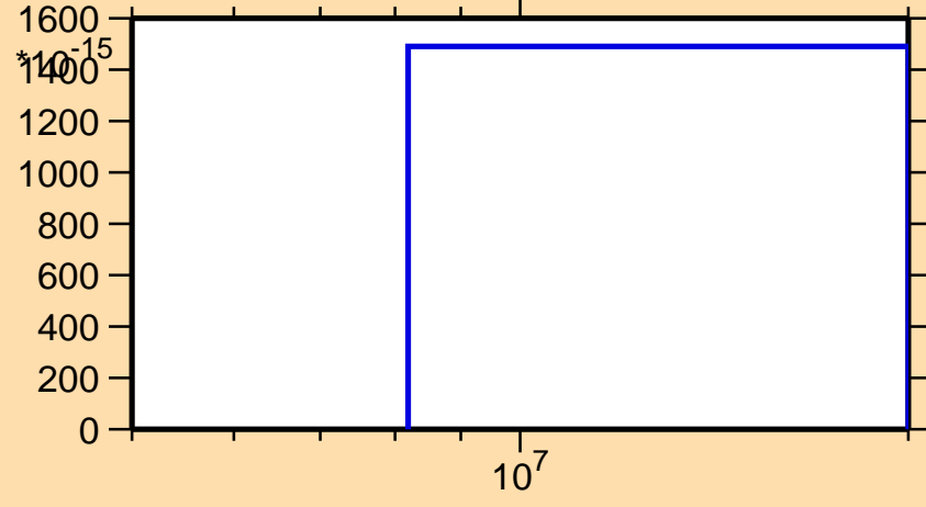
\sigma vs. E for ^{235}\text{U}(n,p\alpha)
