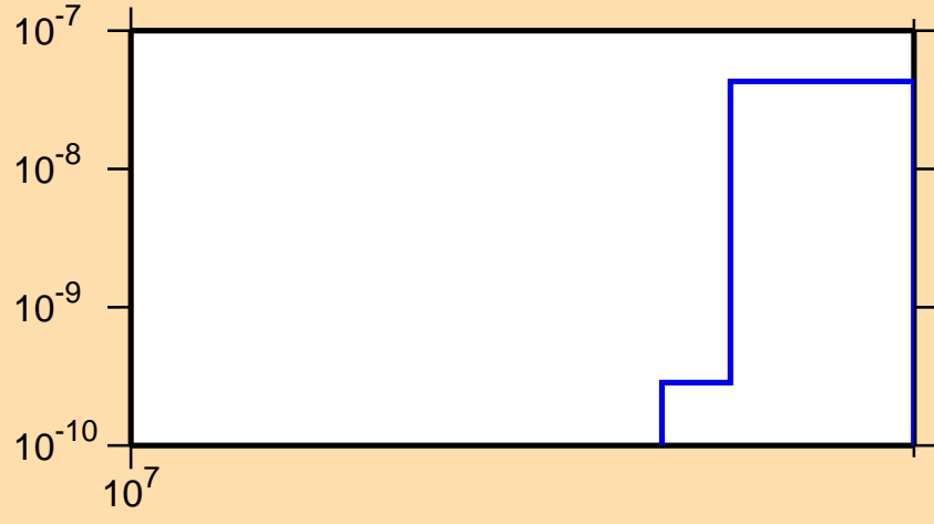
\sigma vs. E for ^{236}\text{U}(n,nd)
