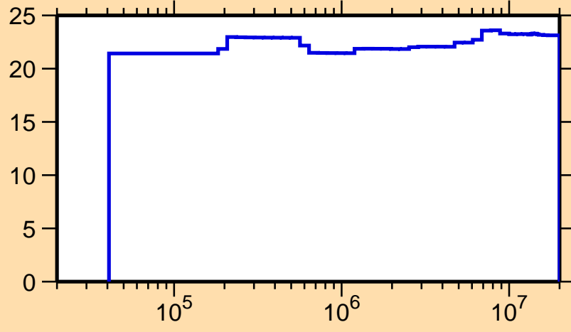
\Delta\sigma/\sigma vs. E for ^{236}\text{U}(n,inel.)
