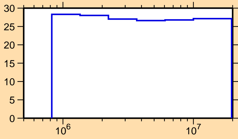
\Delta\sigma/\sigma vs. E for ^{236}\text{U}(n,el.)
