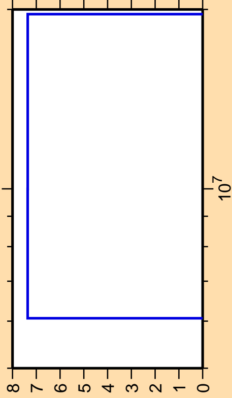
\Delta\sigma/\sigma vs. E for ^{236}\text{U}(n,p)
