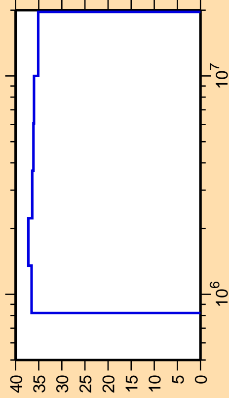
\Delta\sigma/\sigma vs. E for ^{236}\text{U}(n,ncont.)
