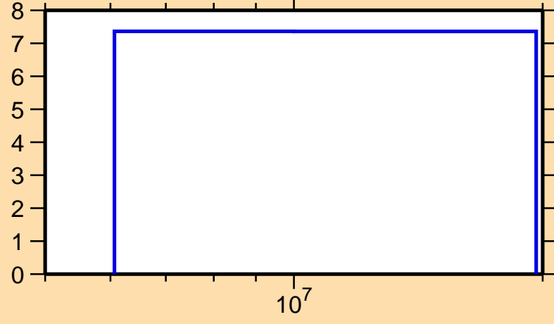
\Delta\sigma/\sigma vs. E for ^{236}\text{U}(n,p)
