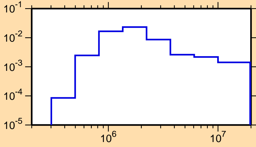
\sigma vs. E for ^{236}\text{U}(n,n_3)
