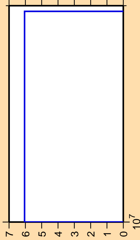
\Delta\sigma/\sigma vs. E for ^{236}\text{U}(n,2np)
