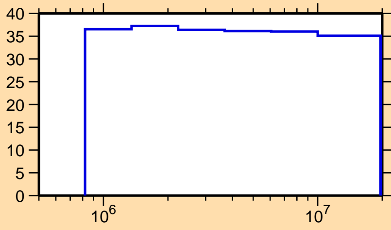
\Delta\sigma/\sigma vs. E for ^{236}\text{U}(n,ncont.)
