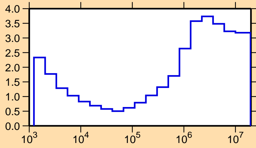
\sigma vs. E for ^{236}\text{U}(n,\text{nonel.})
