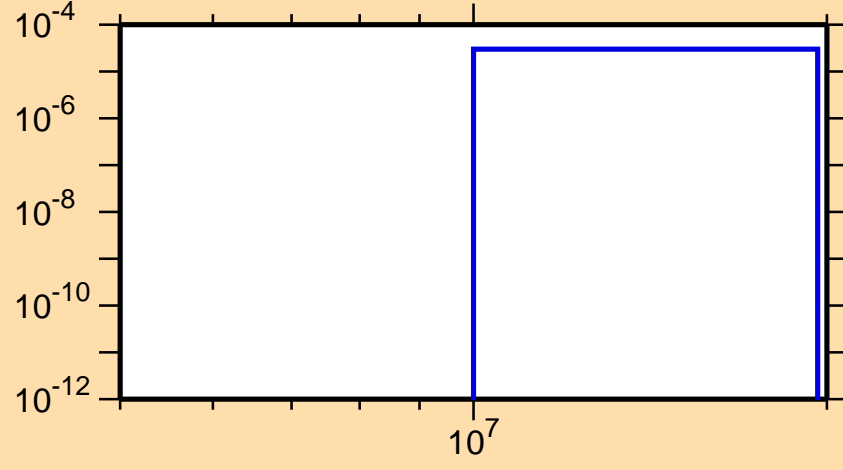
\sigma vs. E for ^{236}\text{U}(n,d)
