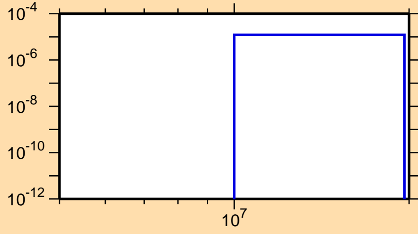
\sigma vs. E for ^{236}\text{U}(n,np)
