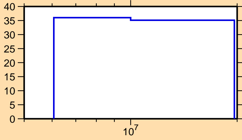
\Delta\sigma/\sigma vs. E for ^{236}\text{U}(n,ncont.)
