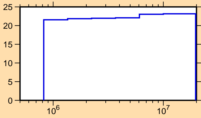
\Delta\sigma/\sigma vs. E for ^{236}\text{U}(n,inel.)
