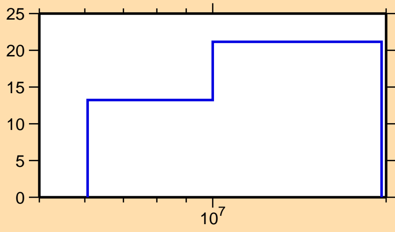
\Delta\sigma/\sigma vs. E for ^{236}\text{U}(n,\gamma)
