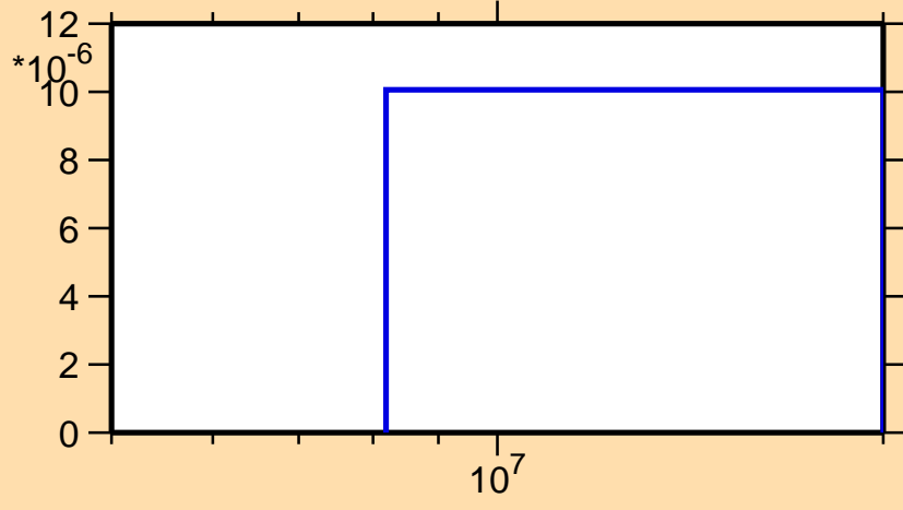
\sigma vs. E for ^{236}\text{U}(n,t)
