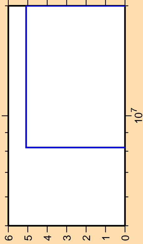
\Delta\sigma/\sigma vs. E for ^{236}\text{U}(n,np)
