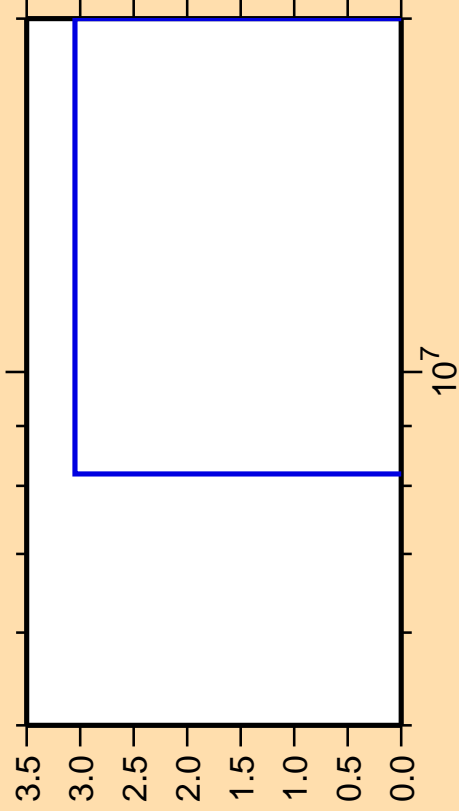
\Delta\sigma/\sigma vs. E for ^{236}\text{U}(n,t)
