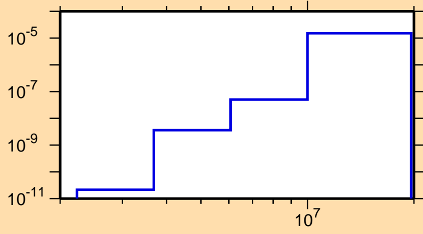
\sigma vs. E for ^{237}\text{U}(n,n\alpha)
