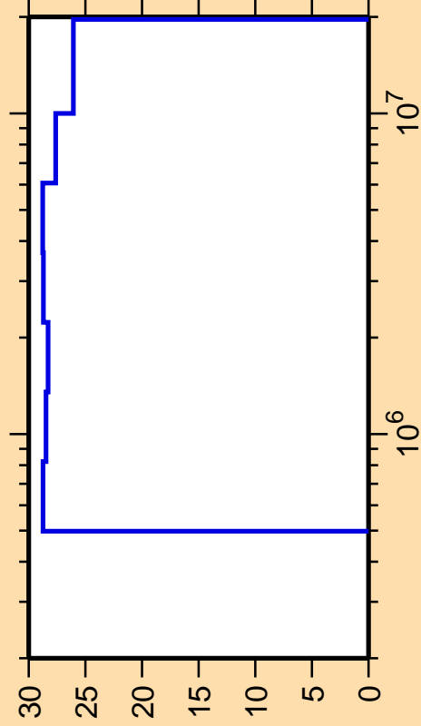
\Delta\sigma/\sigma vs. E for ^{237}\text{U}(n,ncont.)
