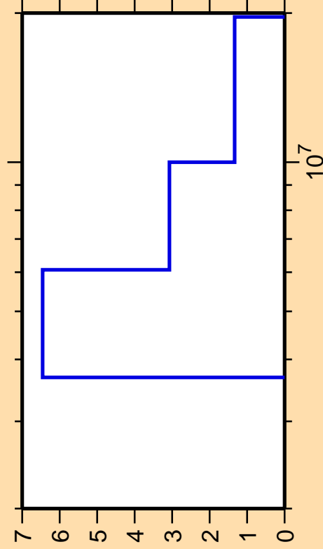
\Delta\sigma/\sigma vs. E for ^{237}\text{U}(n,\alpha)
