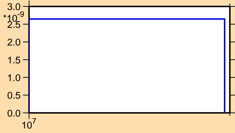
\sigma vs. E for ^{237}\text{U}(n,nd)
