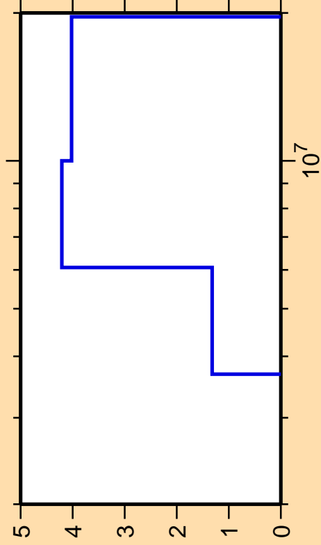
\Delta\sigma/\sigma vs. E for ^{237}\text{U}(n,p)
