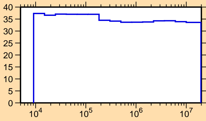
\Delta\sigma/\sigma vs. E for ^{237}\text{U}(n,n_1)
