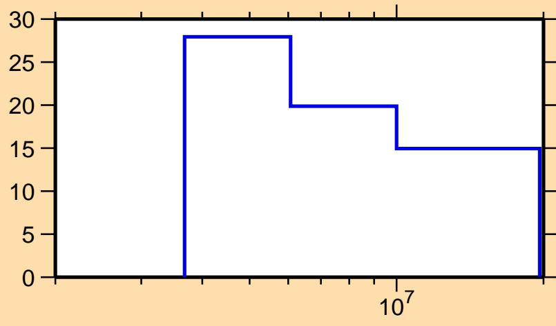
\Delta\sigma/\sigma vs. E for ^{237}\text{U}(n,2n)
