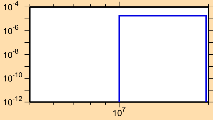
\sigma vs. E for ^{237}\text{U}(n,t)
