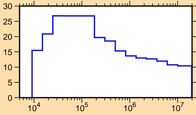
\Delta\sigma/\sigma vs. E for ^{237}\text{U}(n,inel.)
