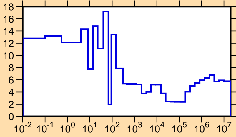
\Delta\sigma/\sigma vs. E for ^{237}\text{U}(n,el.)
