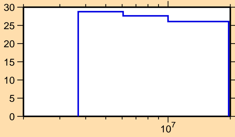
\Delta\sigma/\sigma vs. E for ^{237}\text{U}(n,ncont.)
