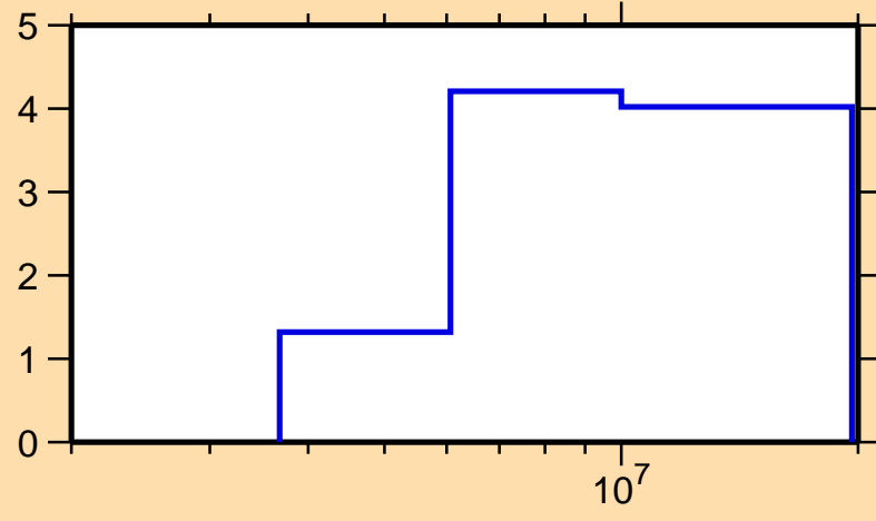
\Delta\sigma/\sigma vs. E for ^{237}\text{U}(n,p)
