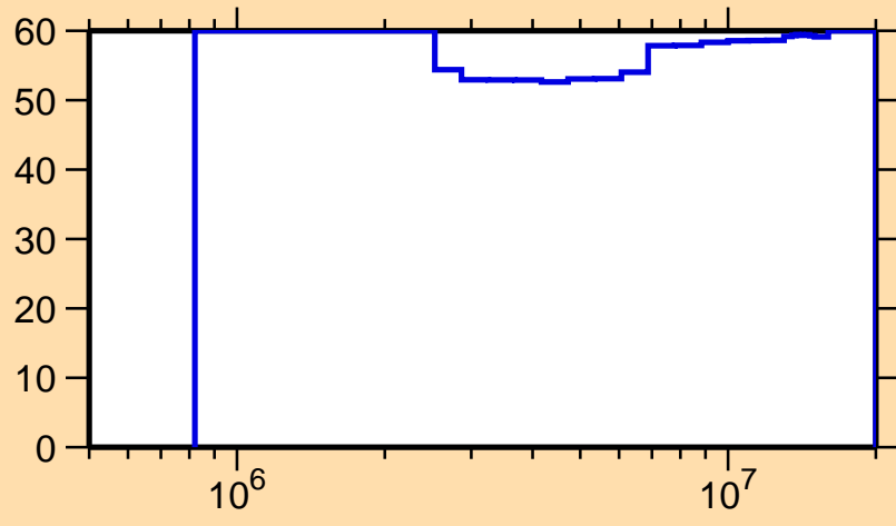
\Delta\sigma/\sigma vs. E for ^{239}\text{U}(n, inel.)
