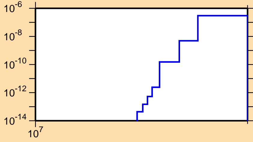
\sigma vs. E for ^{239}\text{U}(n,nt)
