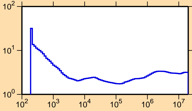
\sigma vs. E for ^{239}\text{U}(n,\text{nonel.})
