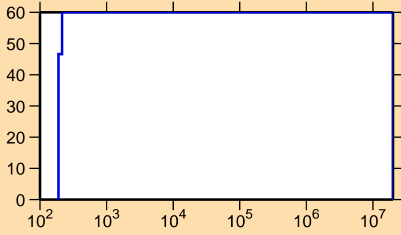
\Delta\sigma/\sigma vs. E for ^{239}\text{U}(n,f)
