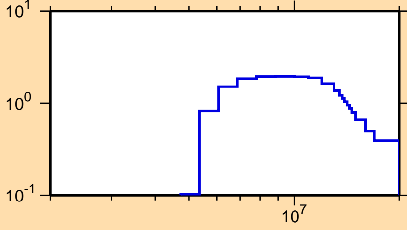
\sigma vs. E for ^{239}\text{U}(n,2n)
