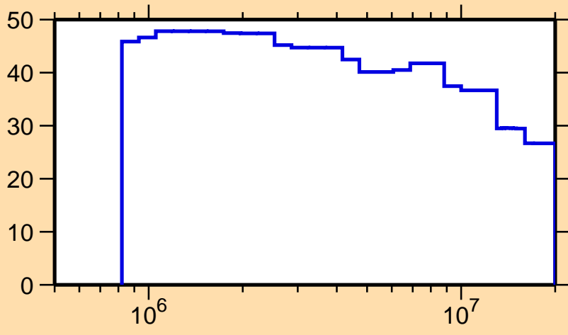
\Delta\sigma/\sigma vs. E for ^{239}\text{U}(n, tot.)
