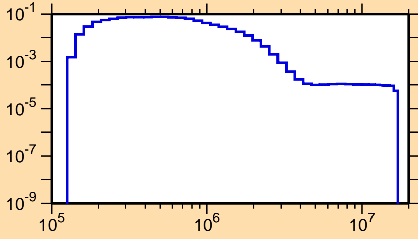
\sigma vs. E for ^{239}\text{U}(n,n_3)
