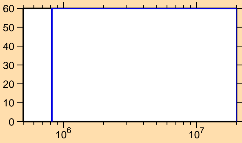
\Delta\sigma/\sigma vs. E for ^{239}\text{U}(n, n_1)
