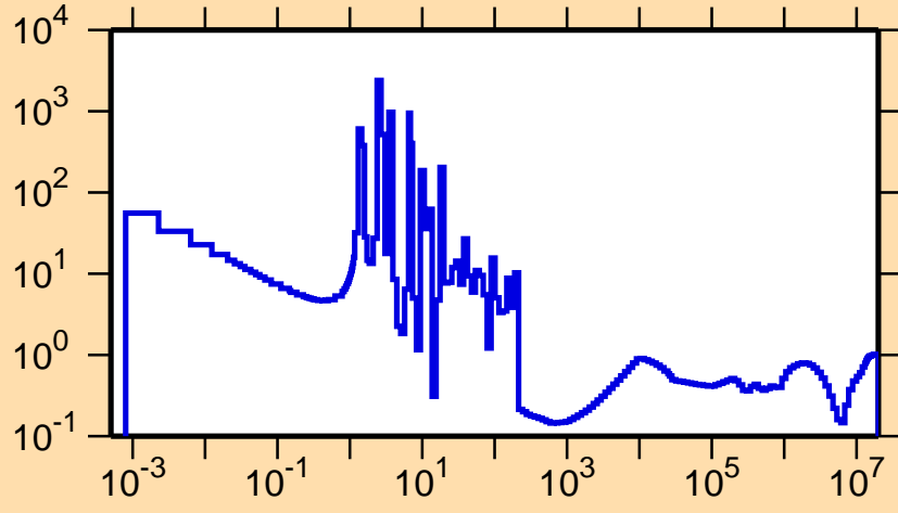
\sigma vs. E for ^{239}\text{U}(n,f)
