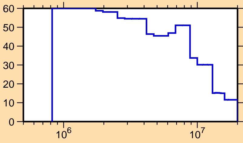
\Delta\sigma/\sigma vs. E for ^{239}\text{U}(n, nonel.)
