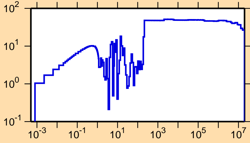
\Delta\sigma/\sigma vs. E for ^{239}\text{U}(n,tot.)
