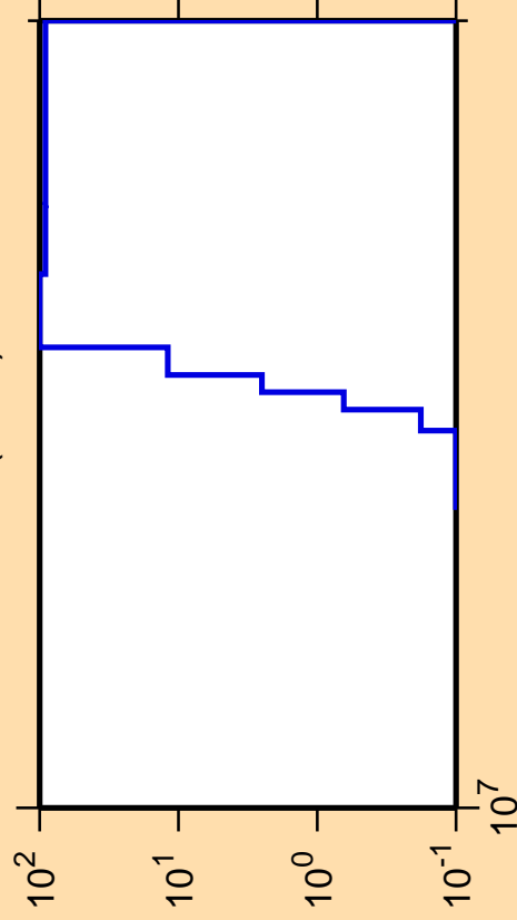
\Delta\sigma/\sigma vs. E for ^{239}\text{U}(n,nd)
