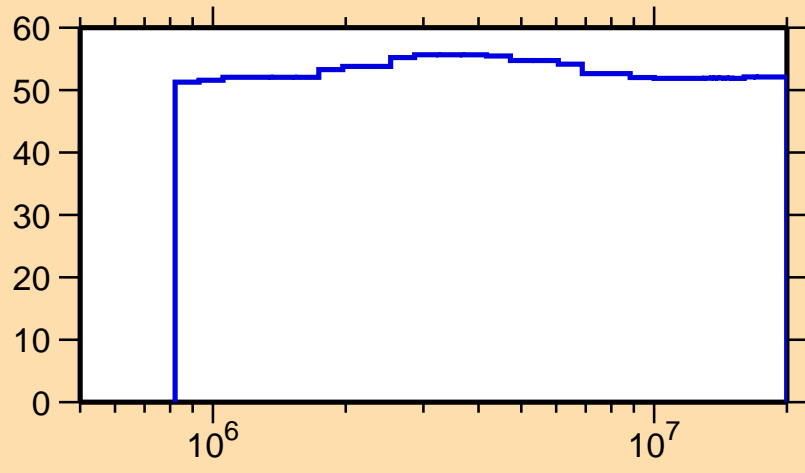
\Delta\sigma/\sigma vs. E for ^{239}\text{U}(n, el.)
