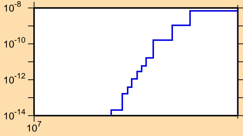
\sigma vs. E for ^{239}\text{U}(n,3n\alpha)
