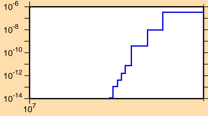
\sigma vs. E for ^{239}\text{U}(n,nd)
