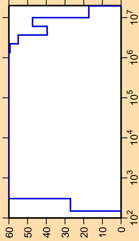
\Delta\sigma/\sigma vs. E for ^{239}\text{U}(n,\text{nonel.})
