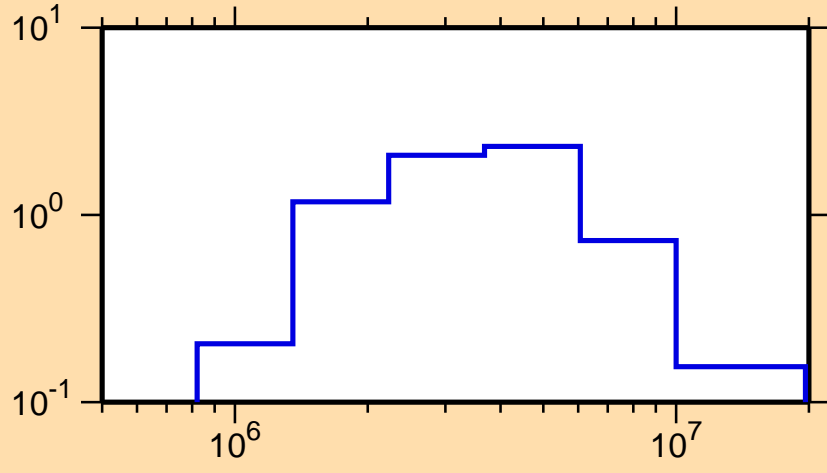
\sigma vs. E for ^{239}\text{U}(n,n\text{cont.})
