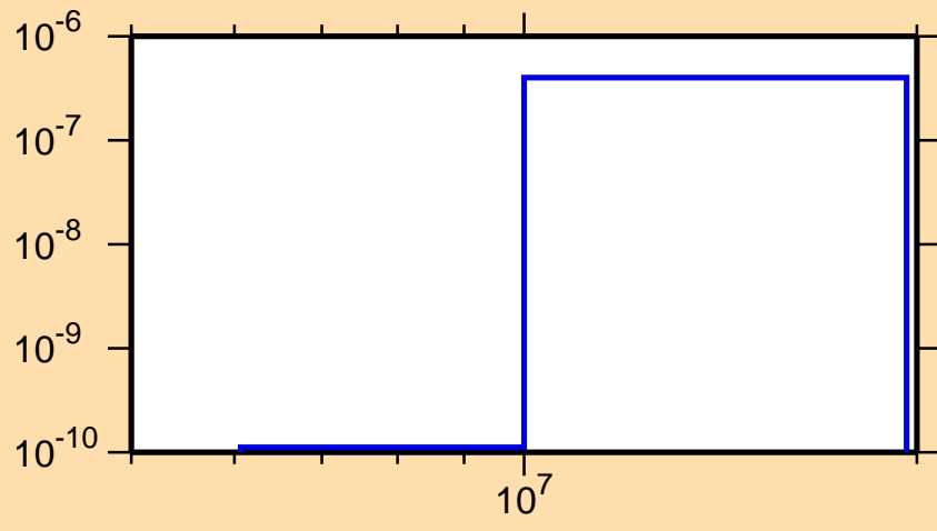
\sigma vs. E for ^{239}\text{U}(n,2n\alpha)
