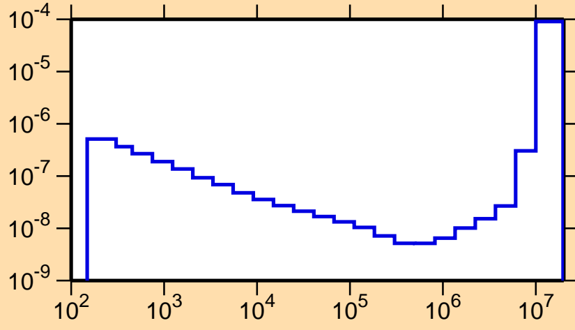
\sigma vs. E for ^{239}\text{U}(n,\alpha)
