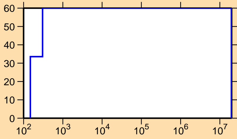
\Delta\sigma/\sigma vs. E for ^{239}\text{U}(n,\gamma)
