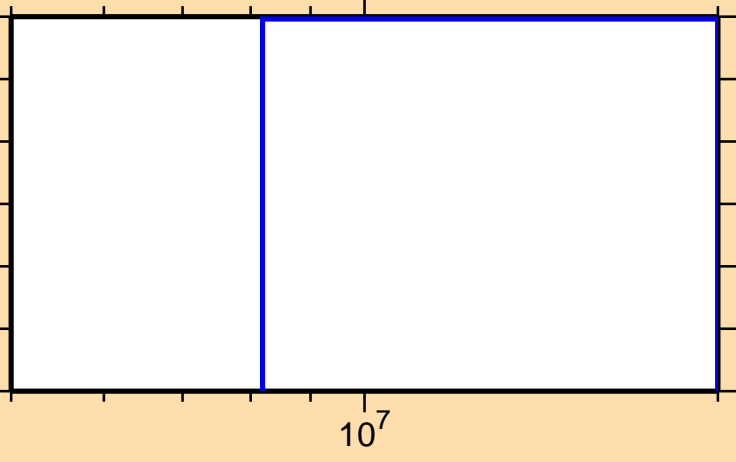
\sigma vs. E for ^{239}\text{U}(n,3n\alpha)
