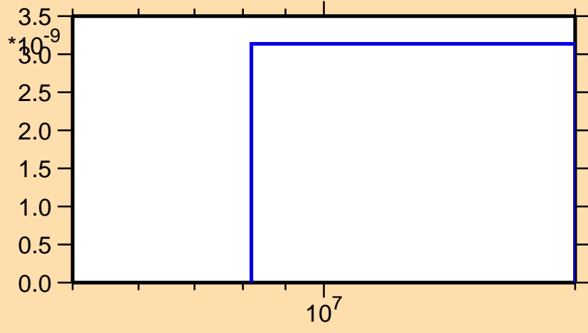
\sigma vs. E for ^{239}\text{U}(n,\text{nd})
