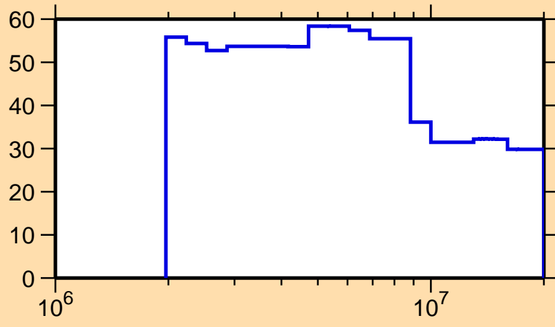
\Delta\sigma/\sigma vs. E for ^{240}\text{U}(n, nonel.)
