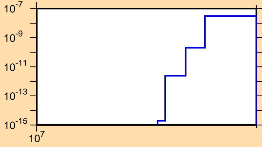
\sigma vs. E for ^{240}\text{U}(n,\text{nd})
