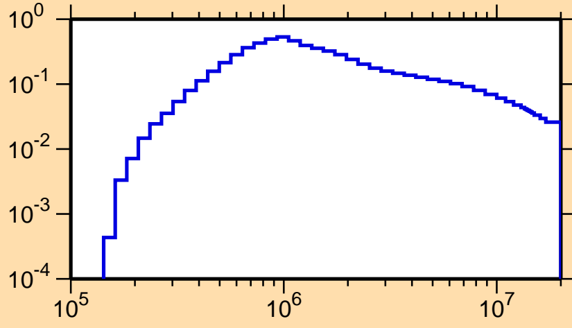
\sigma vs. E for ^{240}\text{U}(n,n_2)
