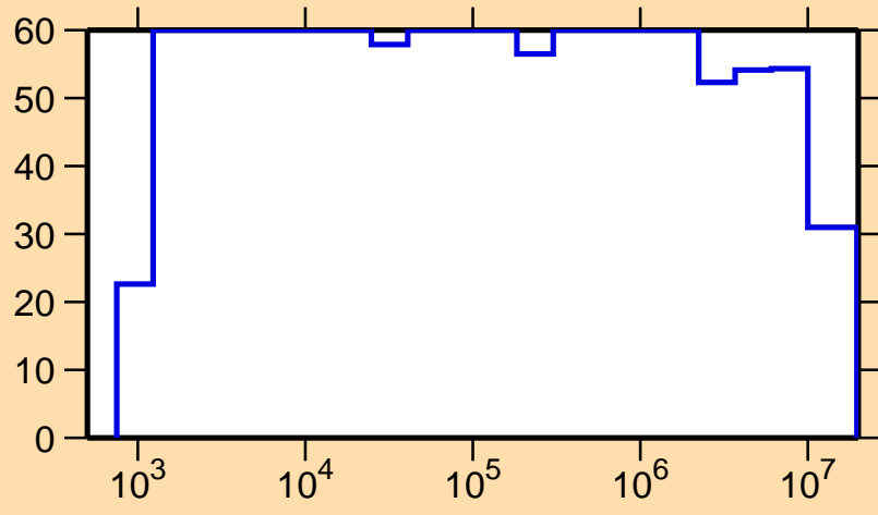
\Delta\sigma/\sigma vs. E for ^{240}\text{U}(n,\text{nonel.})
