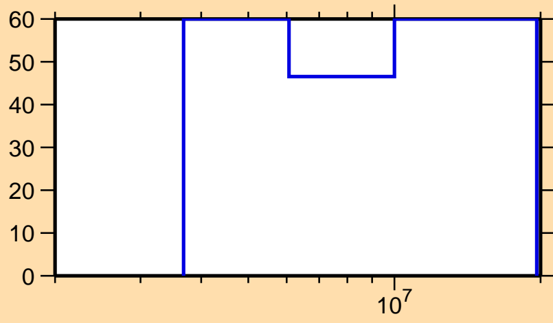
\Delta\sigma/\sigma vs. E for ^{240}\text{U}(n,2n)
