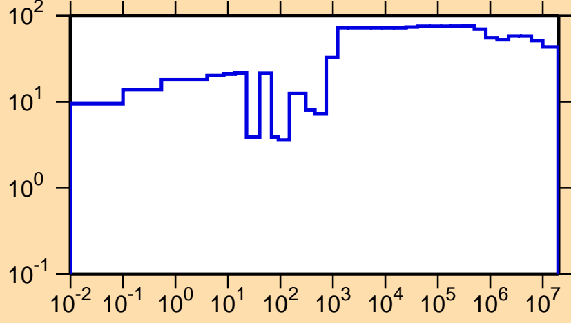
\Delta\sigma/\sigma vs. E for ^{240}\text{U}(n,tot.)
