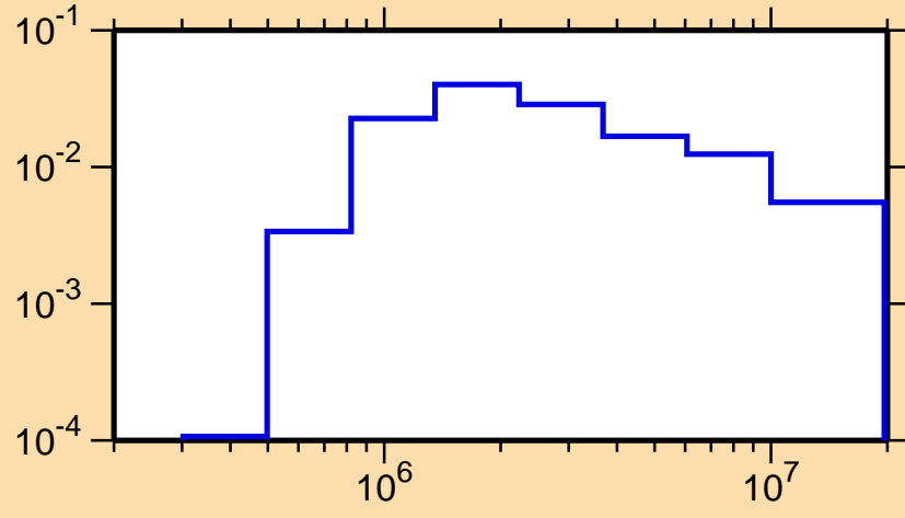
\sigma vs. E for ^{240}\text{U}(n,n_3)
