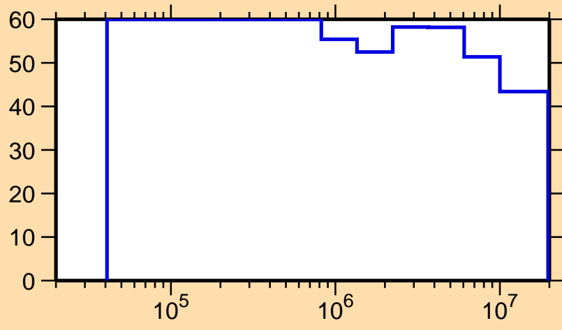
\Delta\sigma/\sigma vs. E for ^{240}\text{U}(n,\text{tot.})
