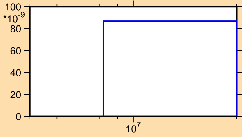
\sigma vs. E for ^{240}\text{U}(n,2n\alpha)
