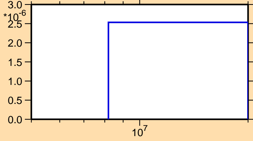
\sigma vs. E for ^{240}\text{U}(n,np)
