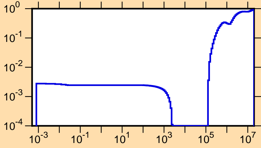
\mu vs. E for ^{241}\text{U}(\text{mt251})
