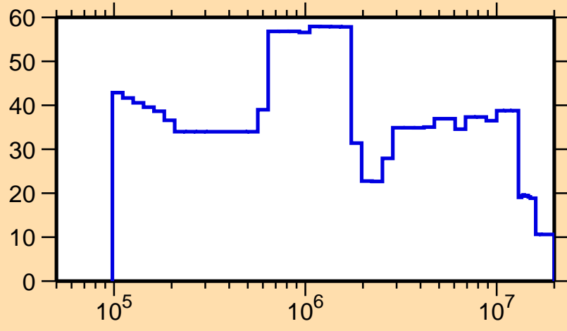
\Delta\sigma/\sigma vs. E for ^{241}\text{U}(n, el.)
