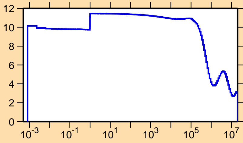
\sigma vs. E for ^{241}\text{U}(n,\text{el.})
