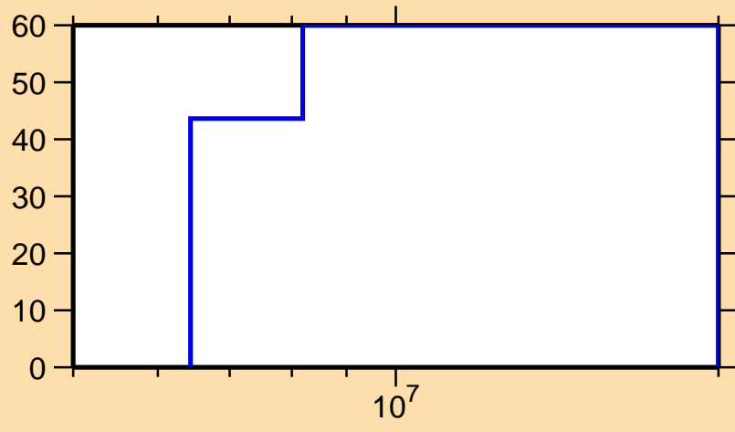
\Delta\sigma/\sigma vs. E for ^{241}\text{U}(n,\gamma)
