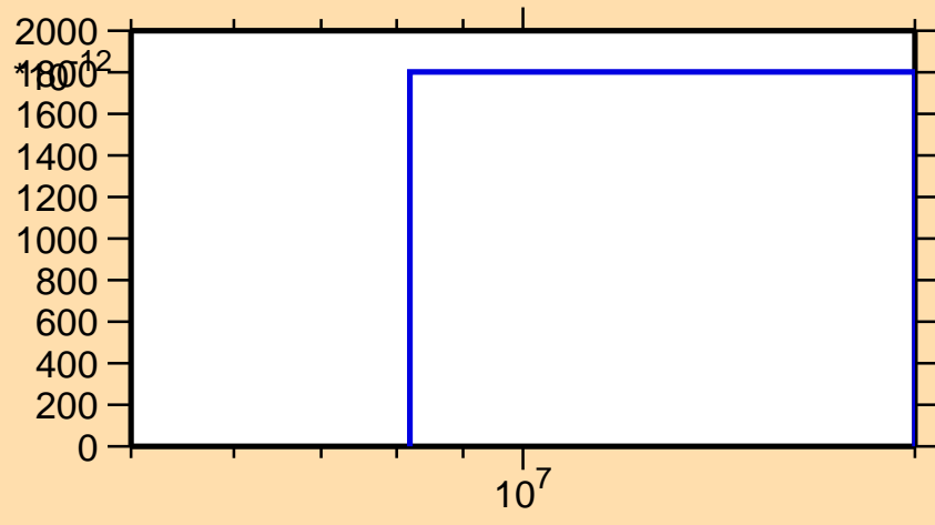
\sigma vs. E for ^{241}\text{U}(n,\text{nd})
