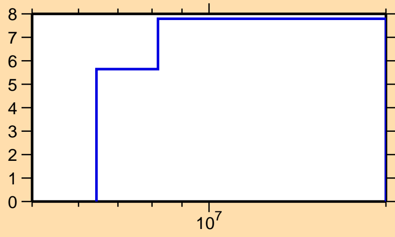
\Delta\sigma/\sigma vs. E for ^{241}\text{U}(n,\text{nonel.})
