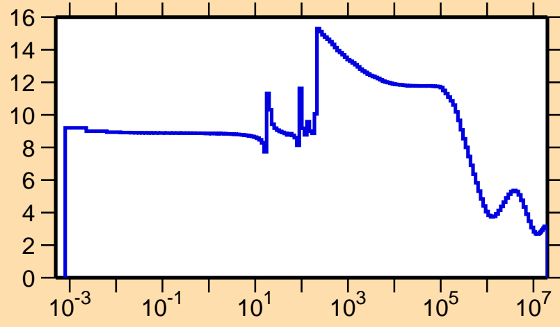
\sigma vs. E for ^{242}\text{U}(n,\text{el.})
