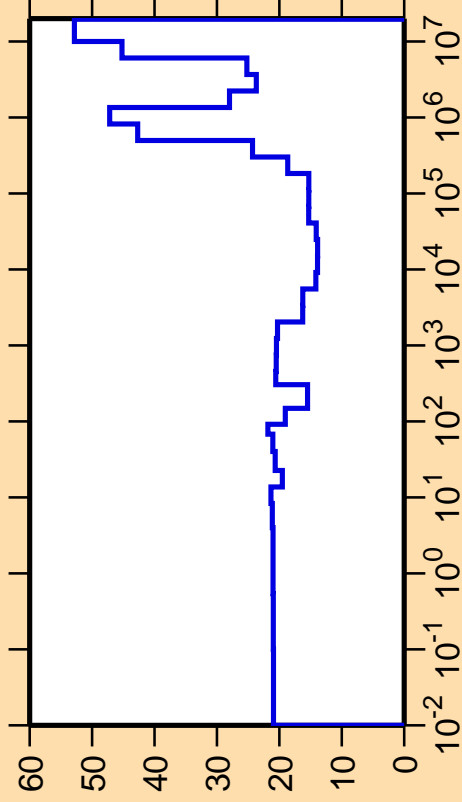
\Delta\sigma/\sigma vs. E for ^{242}\text{U}(n,\text{el.})
