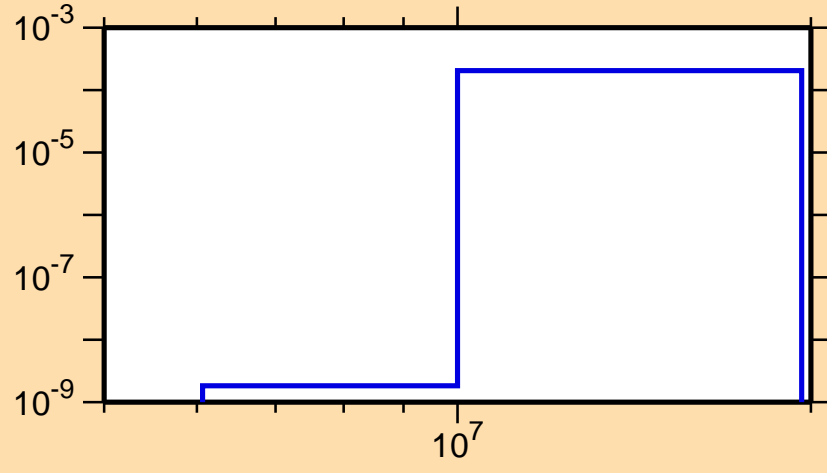
\sigma vs. E for ^{242}\text{U}(n,p)
