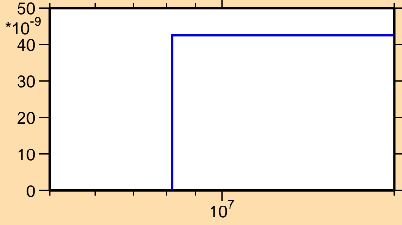
\sigma vs. E for ^{242}\text{U}(n,2n\alpha)
