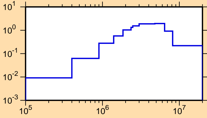
\sigma vs. E for ^{242}\text{U}(n,n\text{cont.})
