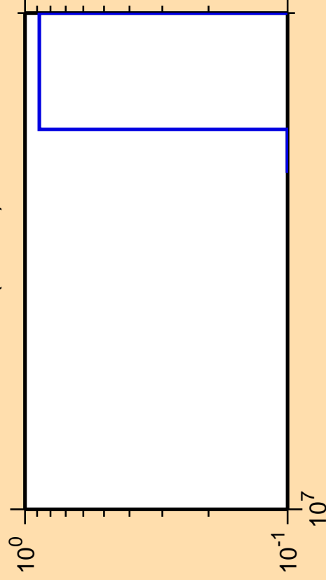
\Delta\sigma/\sigma vs. E for ^{243}\text{U} (mt 11)
