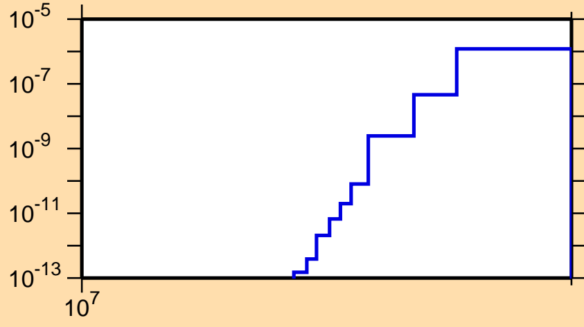
\sigma vs. E for ^{243}\text{U}(n,nd)
