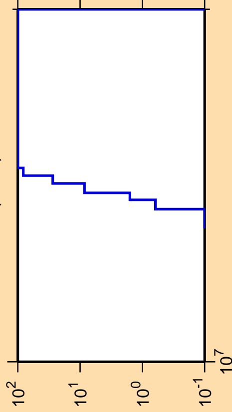
\Delta\sigma/\sigma vs. E for ^{243}\text{U}(n,nd)
