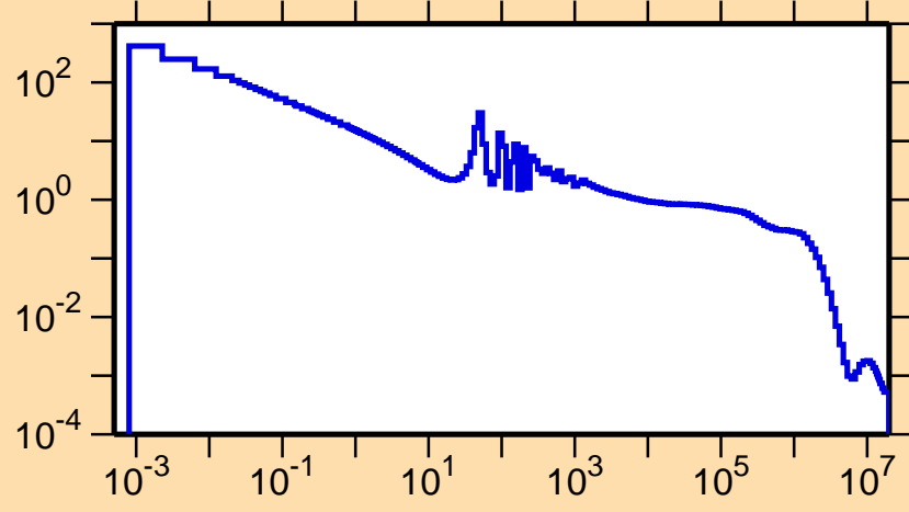
\sigma vs. E for ^{243}\text{U}(n,\gamma)
