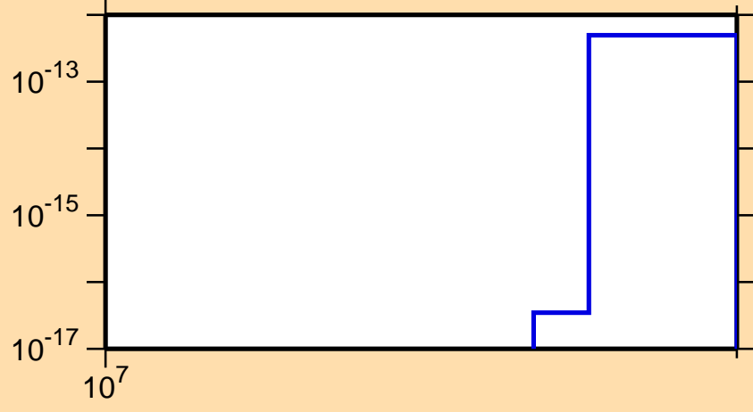
\sigma vs. E for ^{243}\text{U} (mt 11)
