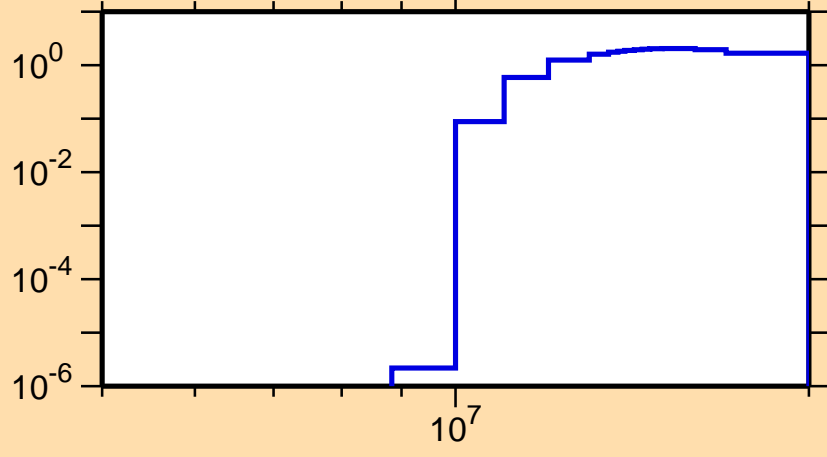
\sigma vs. E for ^{243}\text{U}(n,3n)
