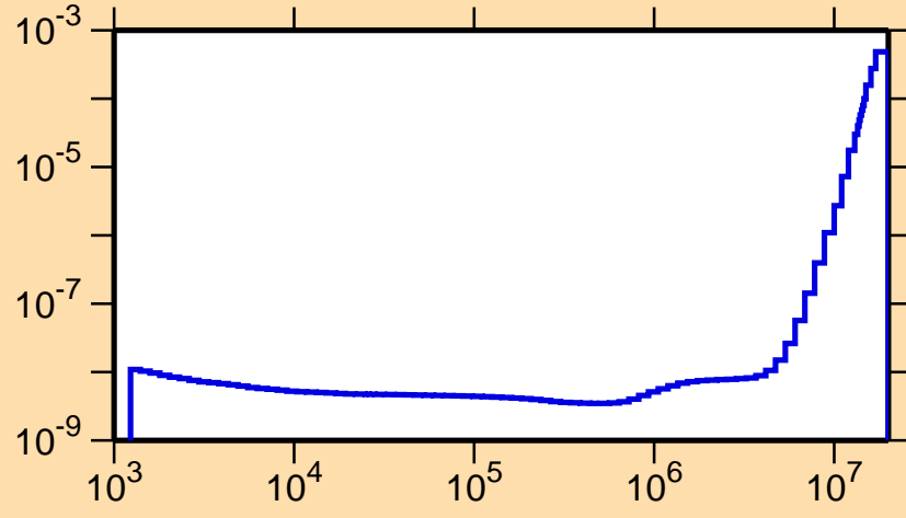
\sigma vs. E for ^{243}\text{U}(n,\alpha)
