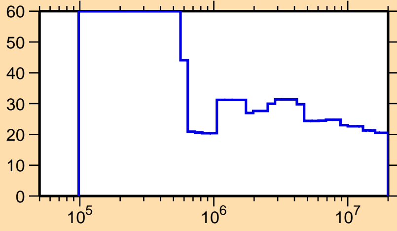
\Delta\sigma/\sigma vs. E for ^{243}\text{U}(n, nonel.)
