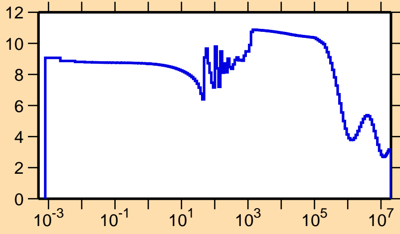
\sigma vs. E for ^{243}\text{U}(n,\text{el.})
