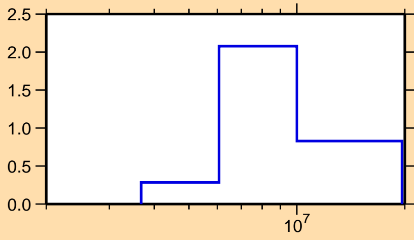
\sigma vs. E for ^{243}\text{U}(n,2n)
