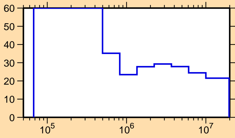
\Delta\sigma/\sigma vs. E for ^{243}\text{U}(n, nonel.)
