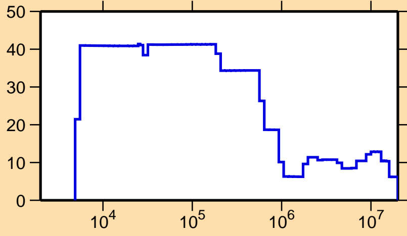
\Delta\sigma/\sigma vs. E for ^{47}\text{V}(n,el.)
