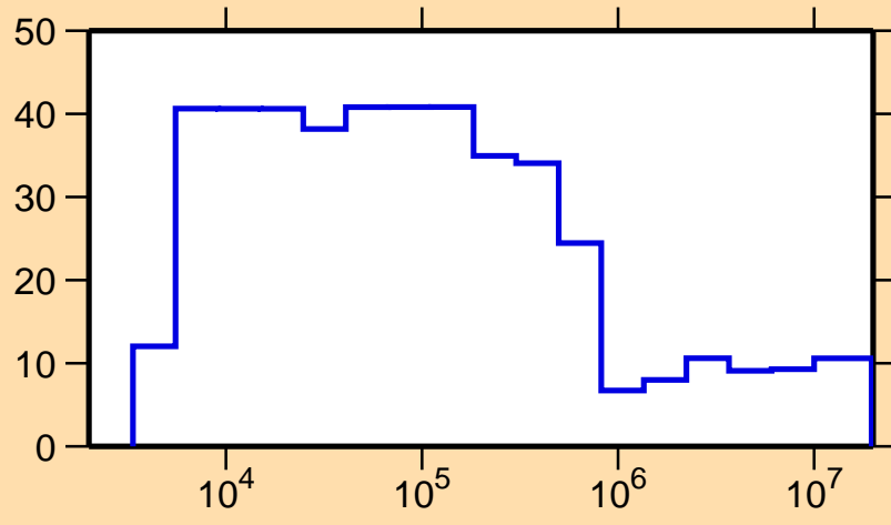
\Delta\sigma/\sigma vs. E for ^{47}\text{V}(n,el.)
