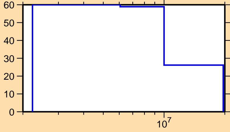
\Delta\sigma/\sigma vs. E for ^{47}\text{V}(n,ncont.)
