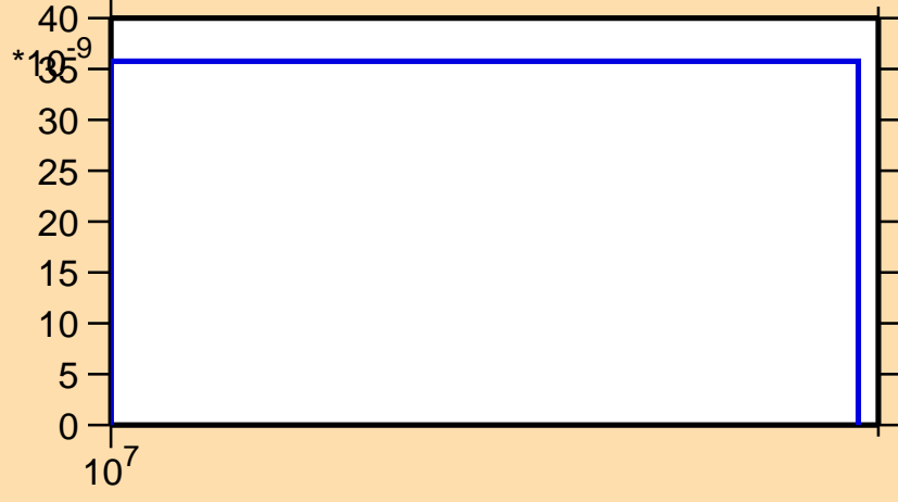
\sigma vs. E for ^{47}\text{V}(n,\text{nd})
