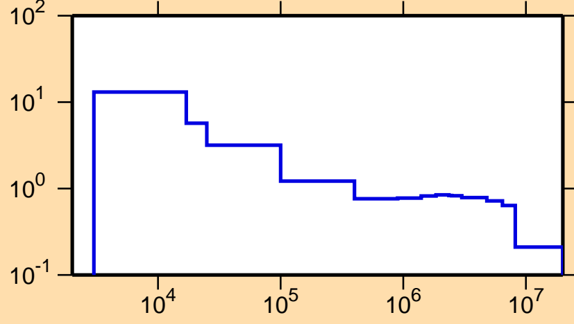
\sigma vs. E for ^{47}\text{V}(n,p)
