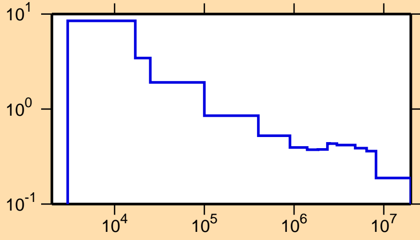
\sigma vs. E for ^{48}\text{V}(n,p)
