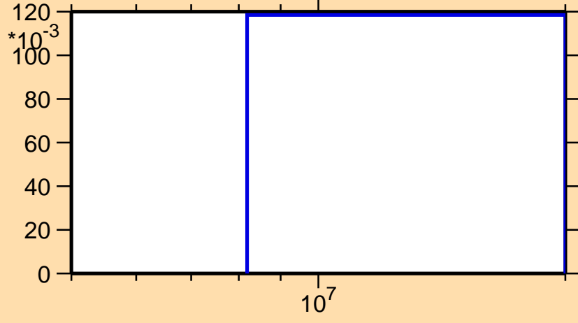
\sigma vs. E for ^{48}\text{V}(n,2n)
