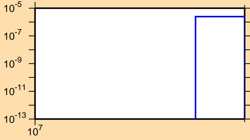
\sigma vs. E for ^{49}\text{V}(n,nd)
