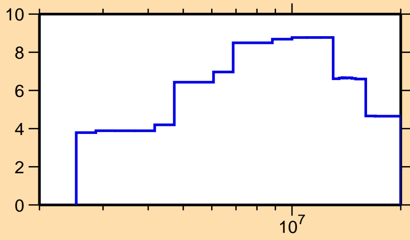
\Delta\sigma/\sigma vs. E for ^{49}\text{V}(n,\text{tot.})
