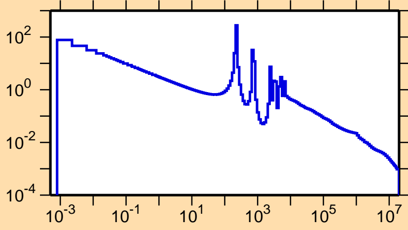
\sigma vs. E for ^{49}\text{V}(n,\gamma)
