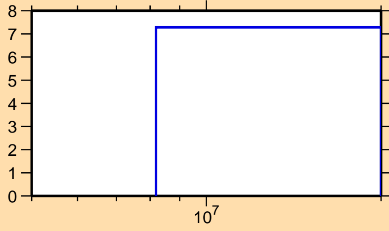
\Delta\sigma/\sigma vs. E for ^{49}\text{V}(n,\text{tot.})
