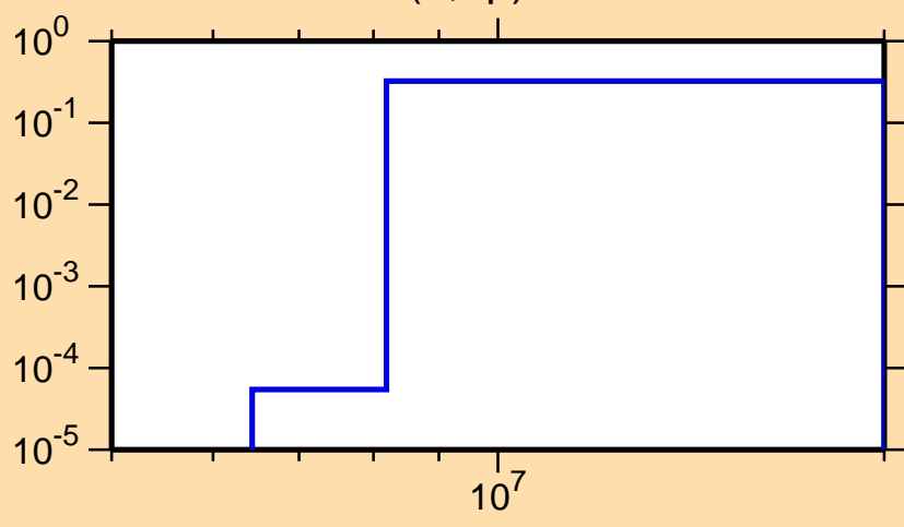
\sigma vs. E for ^{49}\text{V}(n,np)
