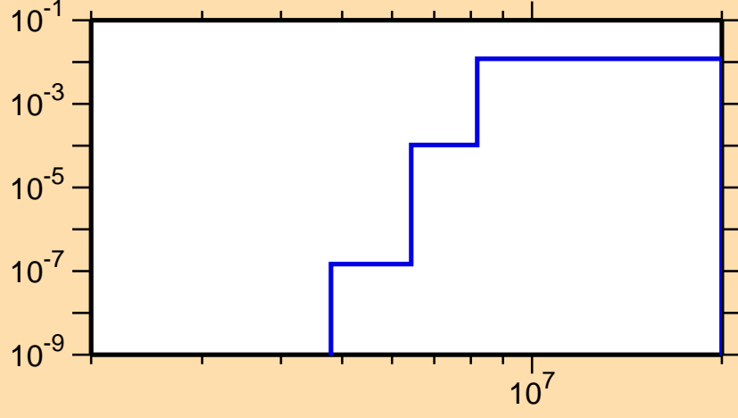
\sigma vs. E for ^{49}\text{V}(n,d)
