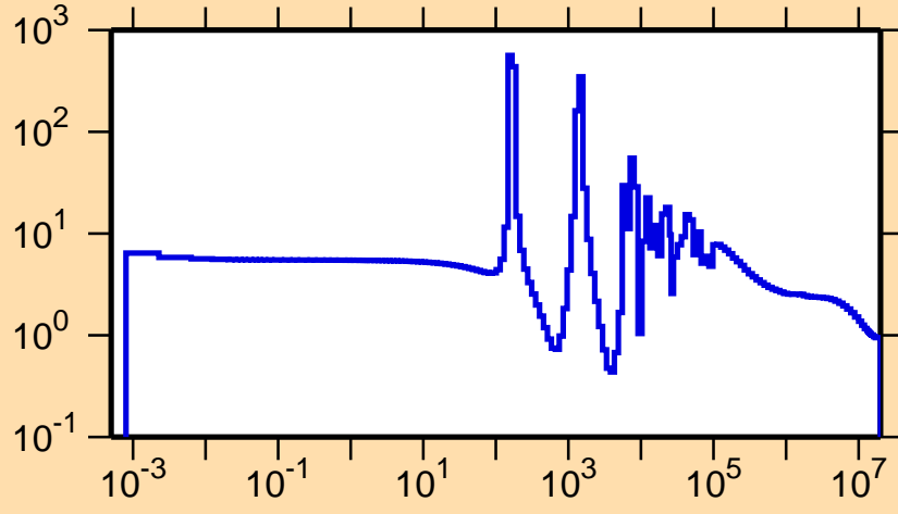
\sigma vs. E for ^{50}\text{V}(n,\text{el.})
