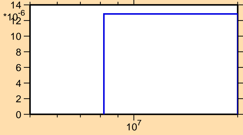
\sigma vs. E for ^{50}\text{V}(n,p\alpha)
