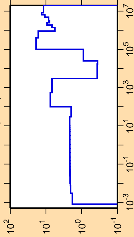
\Delta\sigma/\sigma vs. E for ^{50}\text{V}(n,\text{el.})
