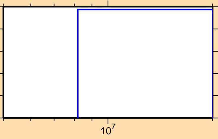
\sigma vs. E for ^{50}\text{V}(n,\text{He3})
