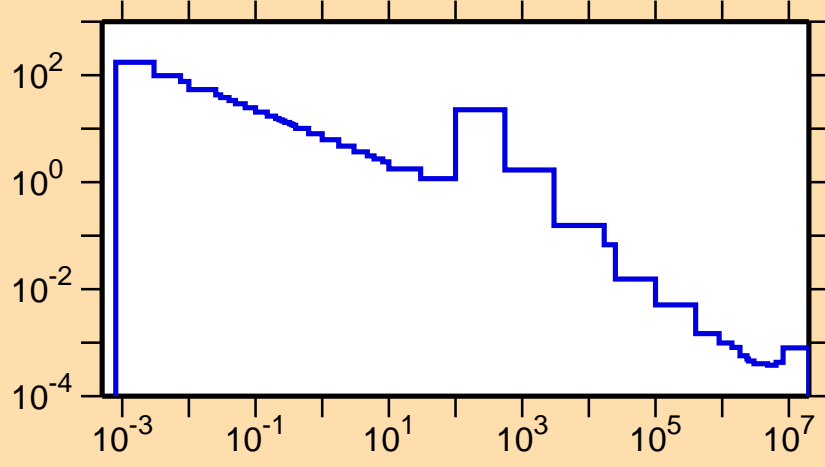
\sigma vs. E for ^{50}\text{V}(n,\gamma)
