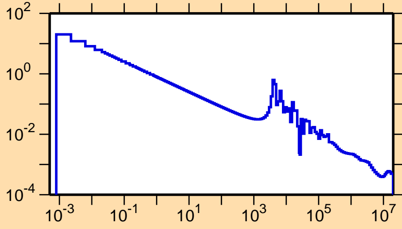
\sigma vs. E for ^{51}\text{V}(n,\gamma)
