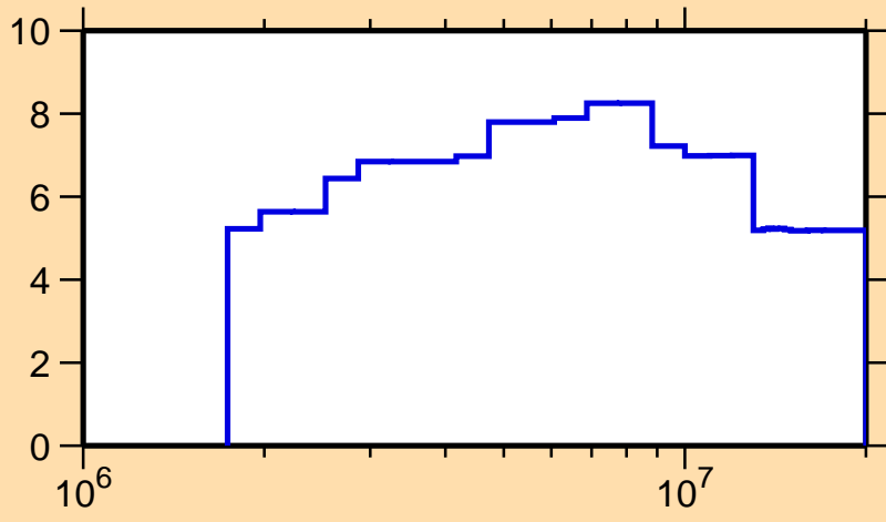
\Delta\sigma/\sigma vs. E for ^{51}\text{V}(n,el.)
