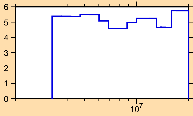
\Delta\sigma/\sigma vs. E for ^{51}\text{V}(n,n\text{onel.})
