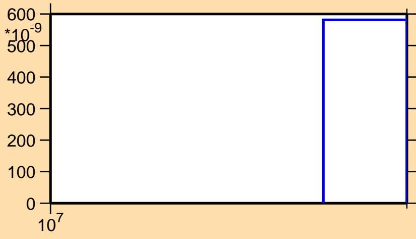
\sigma vs. E for ^{51}\text{V}(n,\text{nd})
