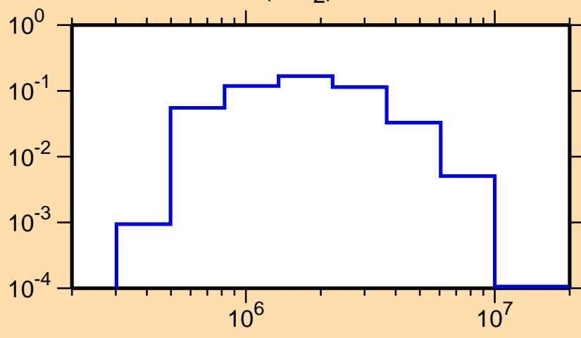
\sigma vs. E for ^{51}\text{V}(n,n_2)
