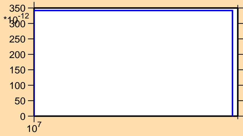
\sigma vs. E for ^{51}\text{V}(n,p\alpha)
