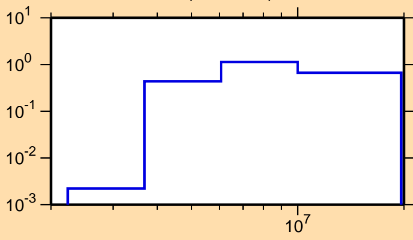
\sigma vs. E for ^{51}\text{V}(n,n\text{cont.})
