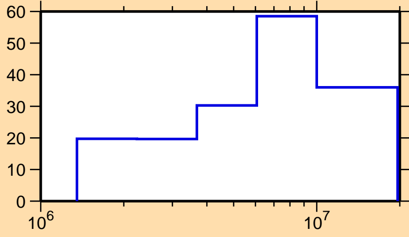
\Delta\sigma/\sigma vs. E for ^{51}\text{V}(n,\gamma)
