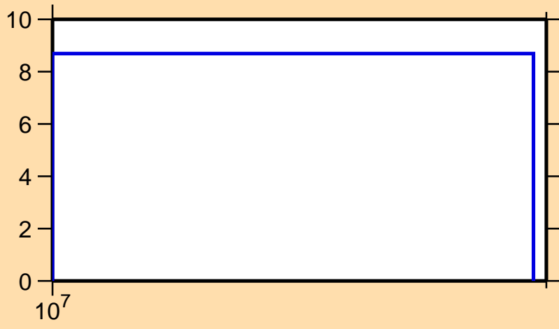
\Delta\sigma/\sigma vs. E for ^{51}\text{V}(n,2n)
