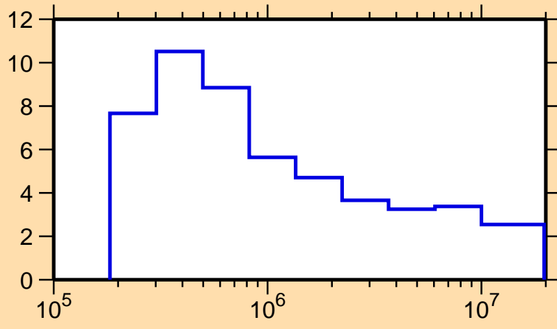
\Delta\sigma/\sigma vs. E for ^{51}\text{V}(n,\text{tot.})
