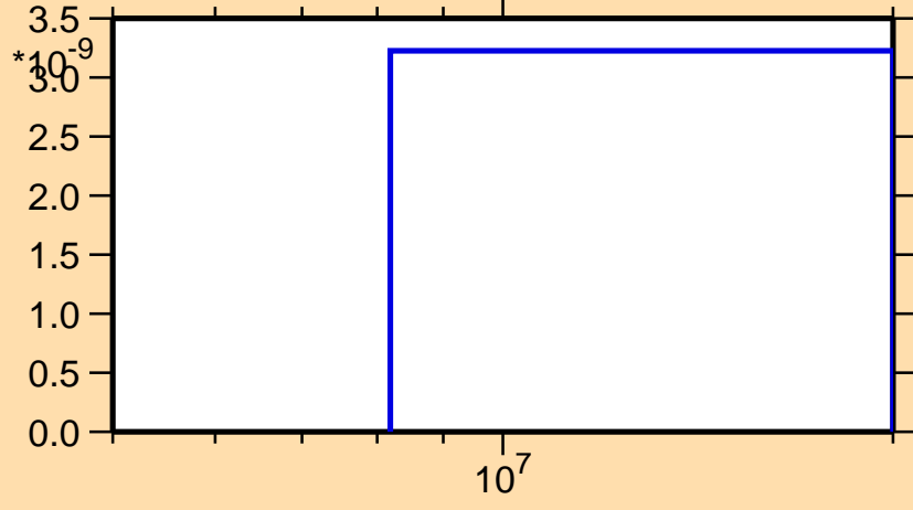
\sigma vs. E for ^{51}\text{V}(n,\text{He}3)
