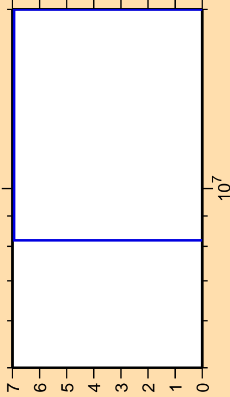
\Delta\sigma/\sigma vs. E for ^{51}\text{V}(n,\alpha)
