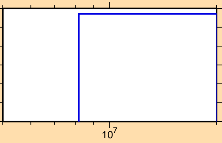
\sigma vs. E for ^{51}\text{V}(n,n\alpha)
